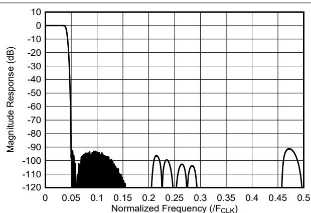
図 7-24. 12x Interpolation Filter Response
