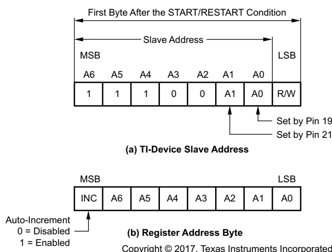
Figure 20. DIX4192 Slave Address and Register Address Byte Definitions
