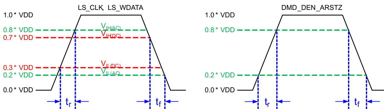
図 6-3. LPSDR Input Rise and Fall Slew Rate
