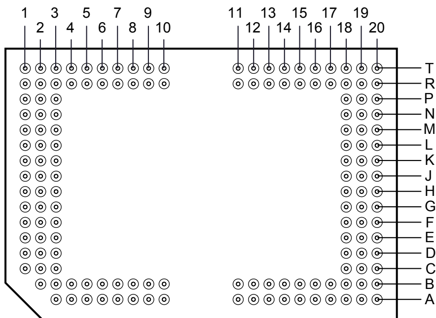
✎ 4-1. FYN Package 149-Pin PGA Bottom View
