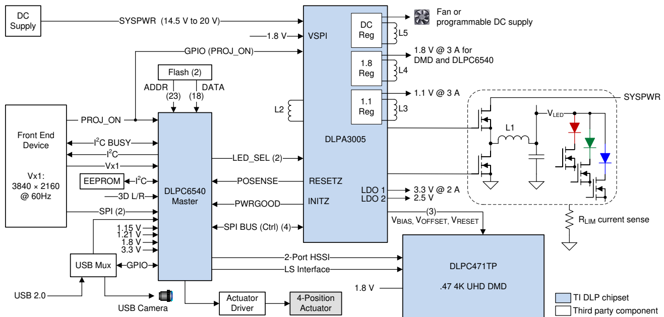
図 8-1. Typical 4K UHD LED Application Diagram
