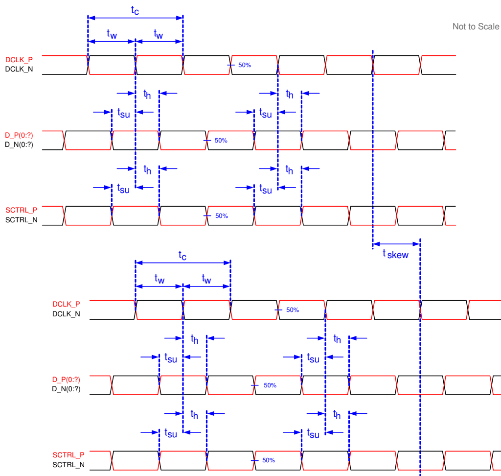
図 5-6. Timing Requirements
