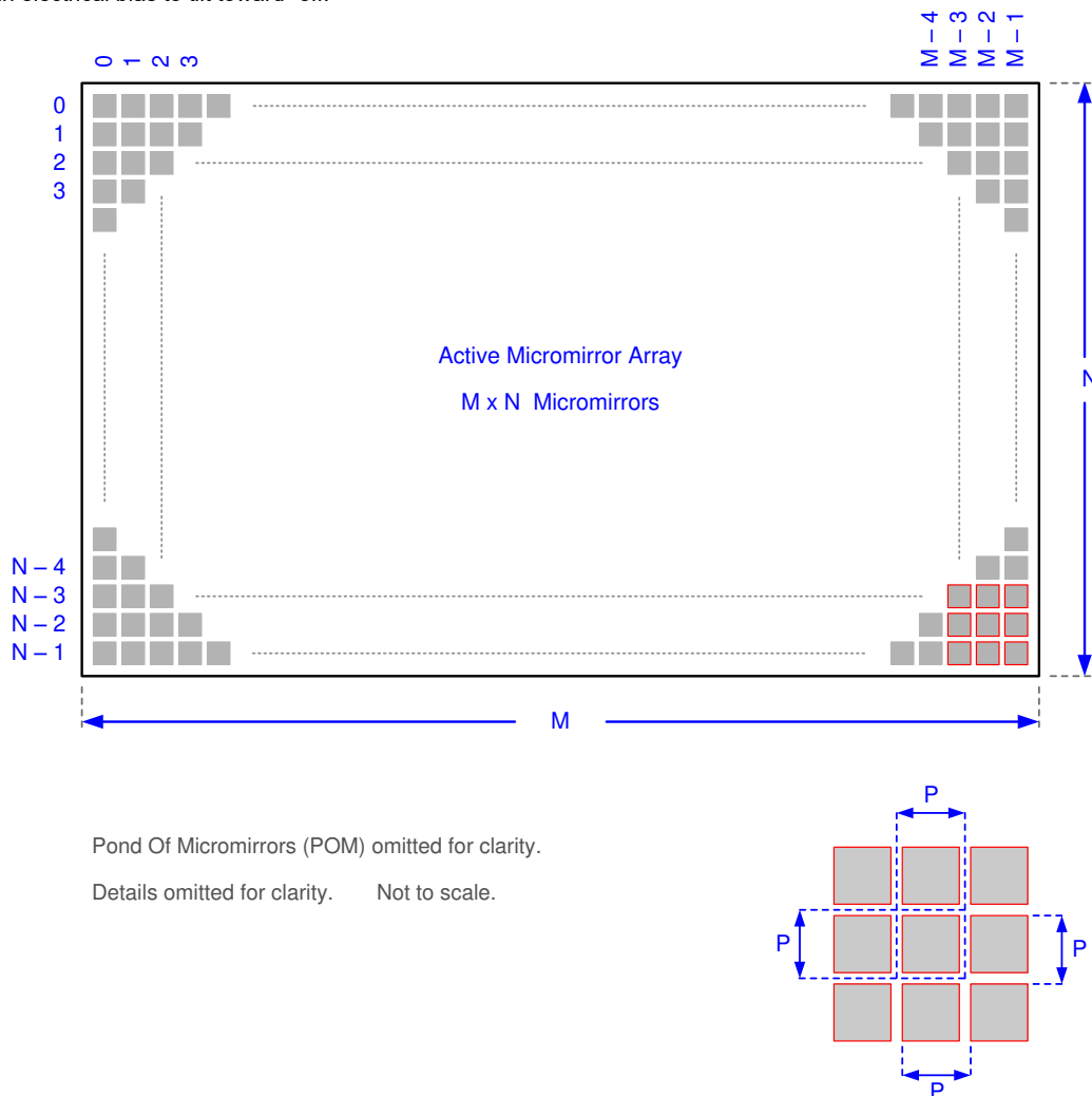
図 5-8. Micromirror Array Physical Characteristics
