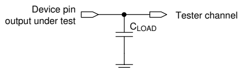
FIG 6-4. Test Load Circuit for Output Propagation Measurement
