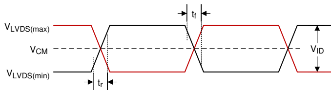
図 6-5. LVDS Waveform Requirements
