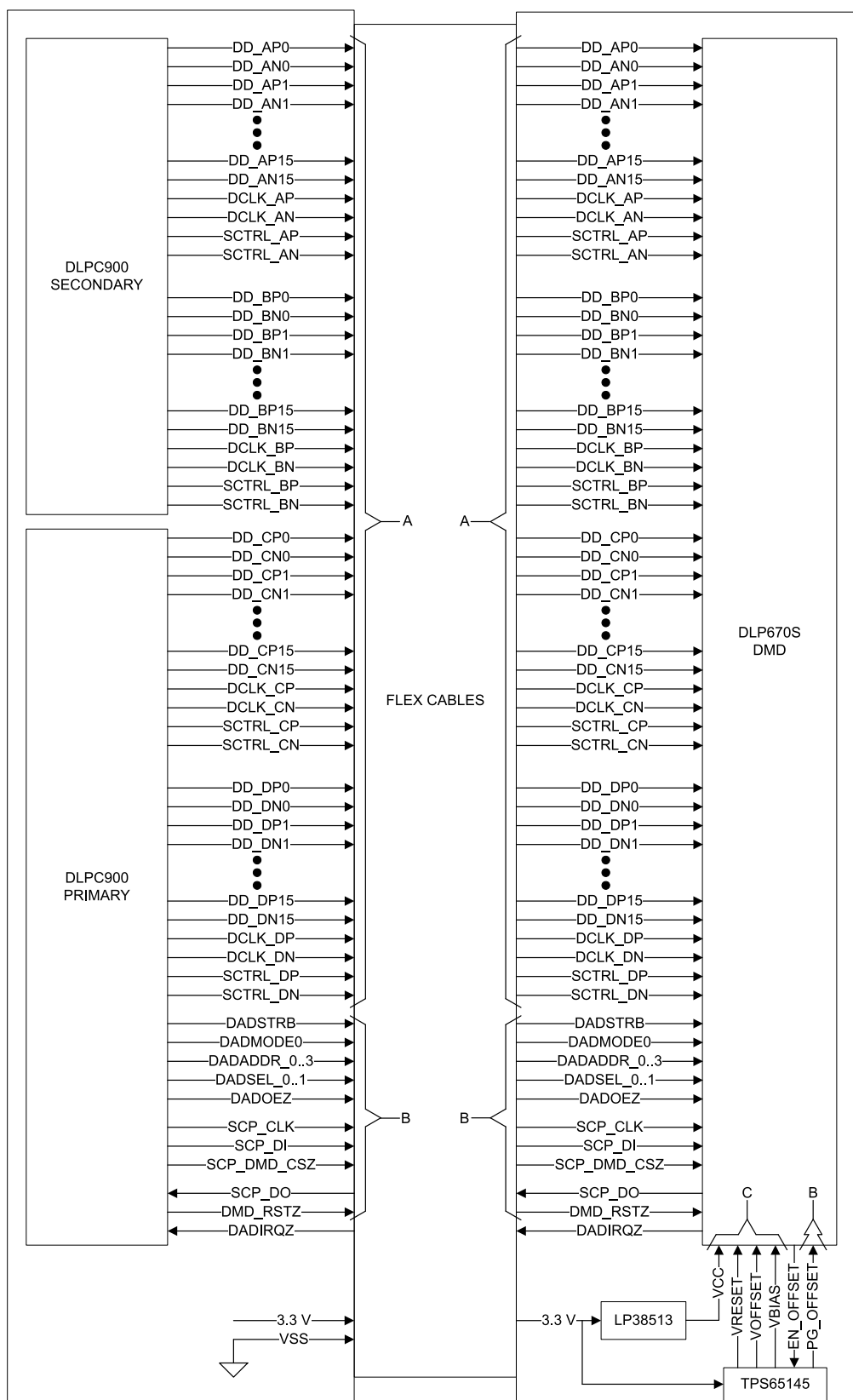
10-1. DLP670S DMD System Connections
