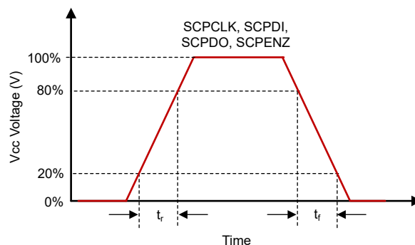
FIG 6-3. SCP Requirements for Rise and Fall
