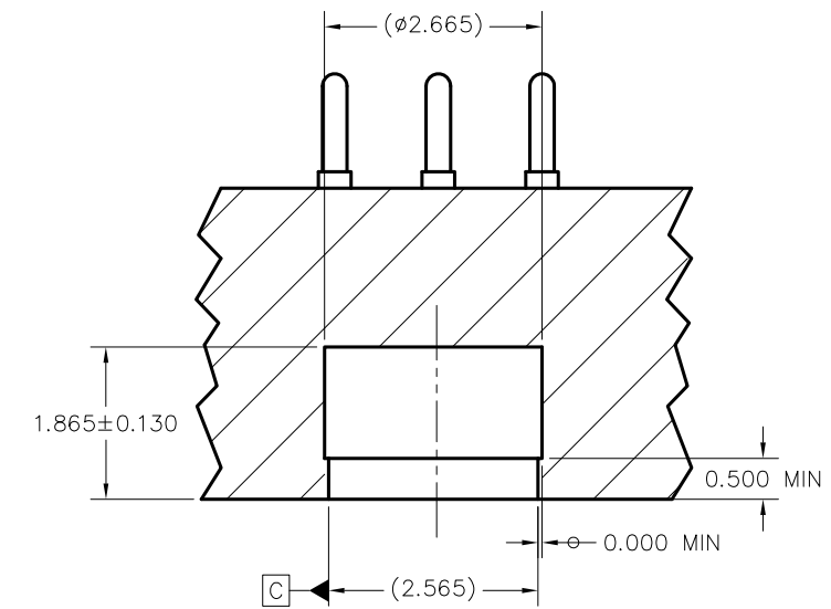
SECTION D-D DATUM C SCALE 16/1
