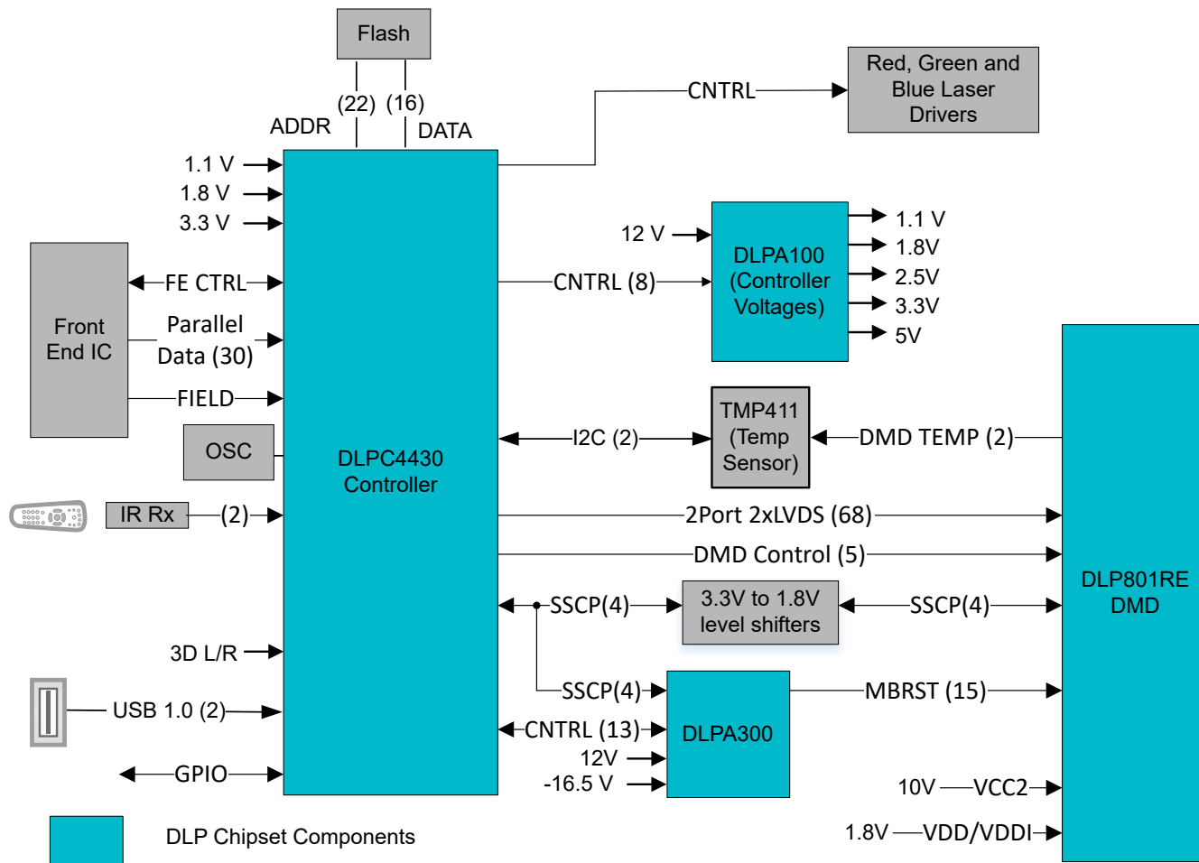
図 8-1. Typical WUXGA RGB Laser Application
