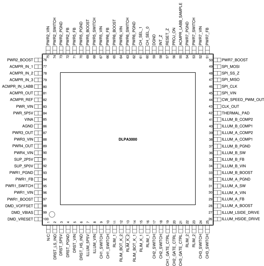
6-1. PFD Package 100-Pin HTQFP Top View
