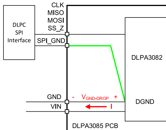
Figure 7-6. SPI Connections
