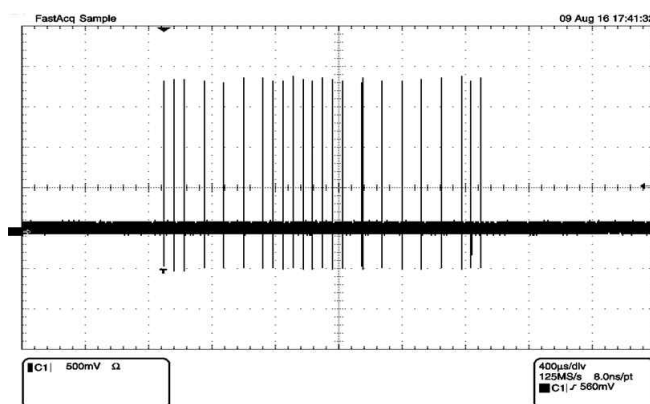
6-11. Auto-Negotiation FLP
