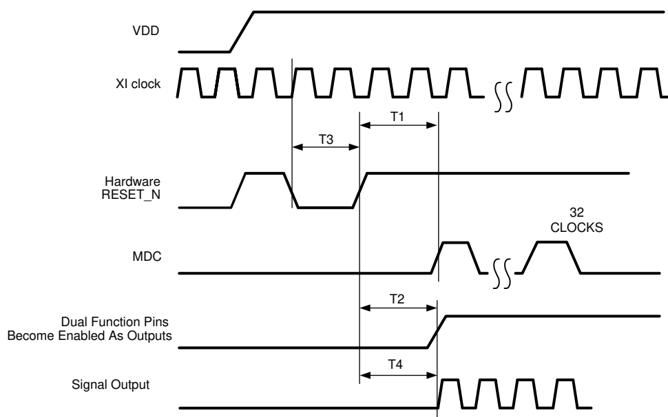
FIG 6-2. Reset Timing
