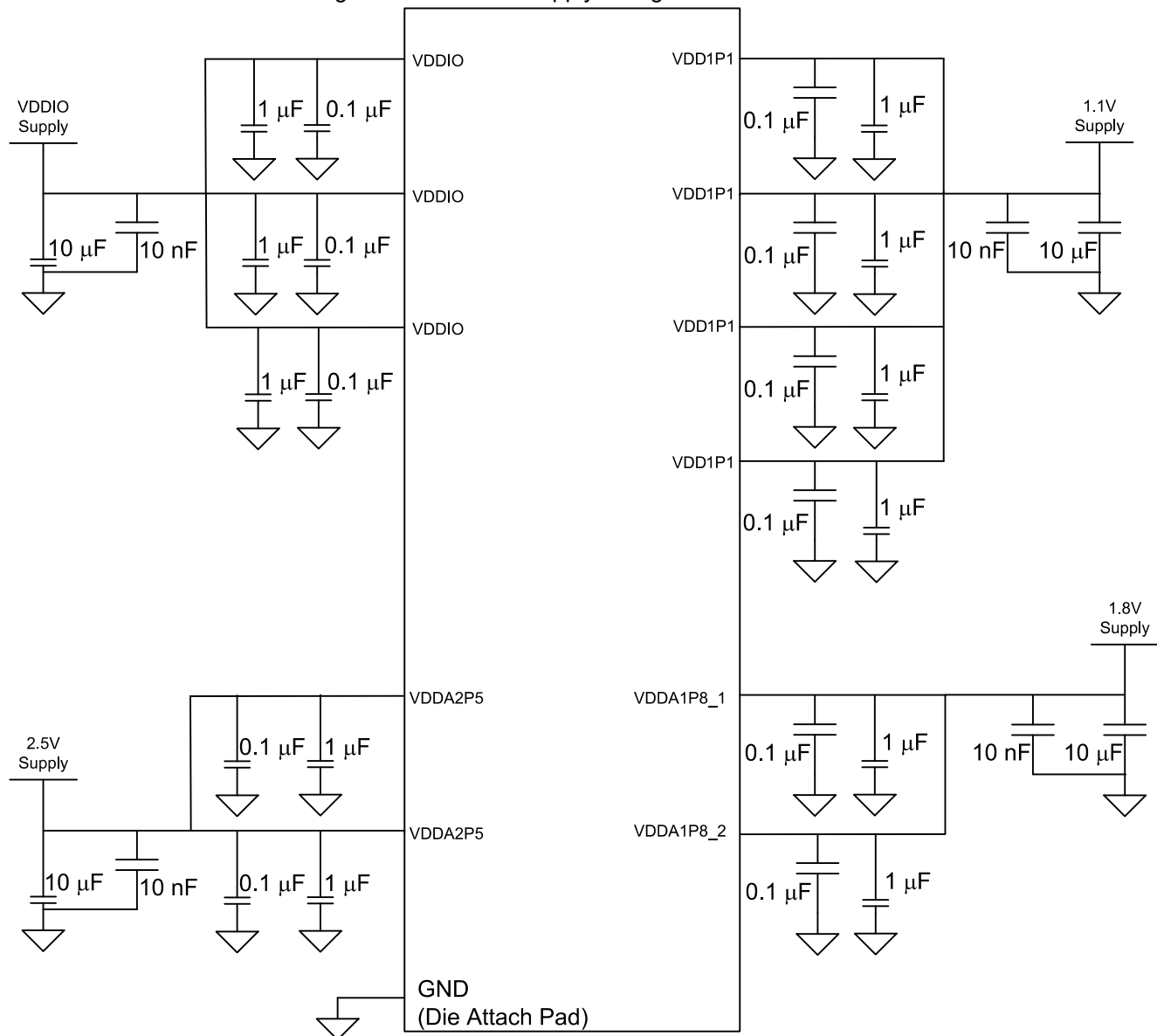
Figure 9-3. Three-Supply Configuration
