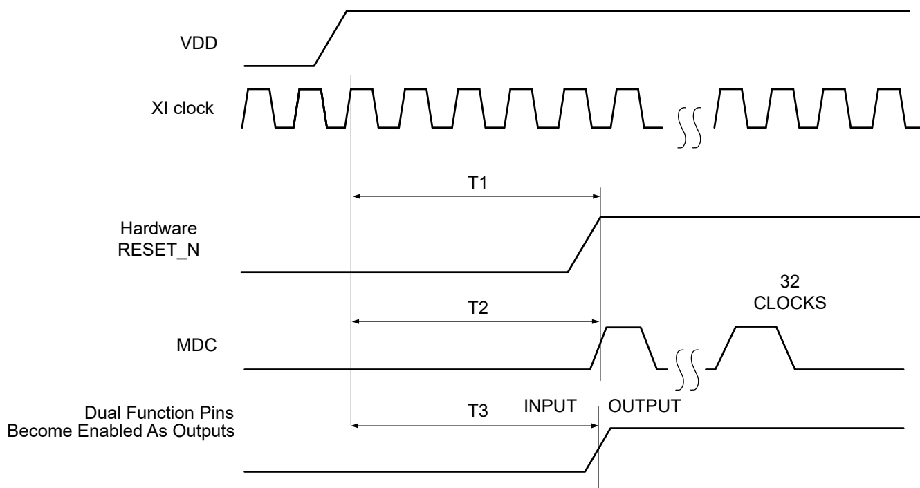
FIG 6-1. Power-Up Timing
