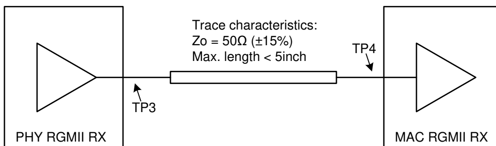
FIG 7-3. RGMII RX Requirements
