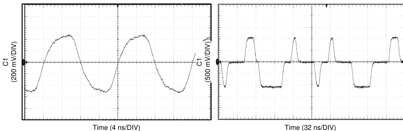
6-8. 1000Base-T Test Mode 2 Signal
