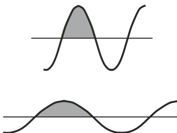
8-30. BEMF Integration
