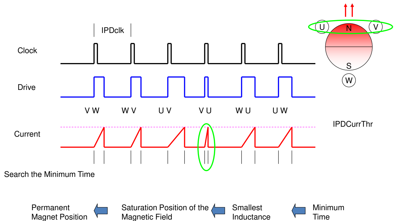
Figure 8-14. IPD Function
