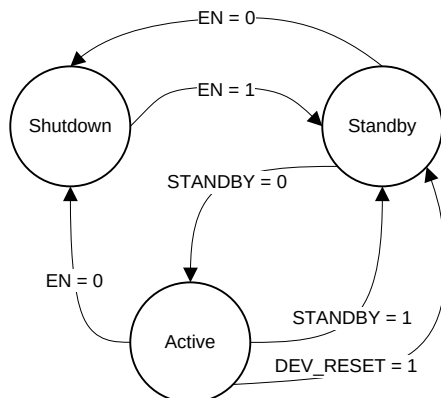
Figure 17. Power-State Transition Diagram
