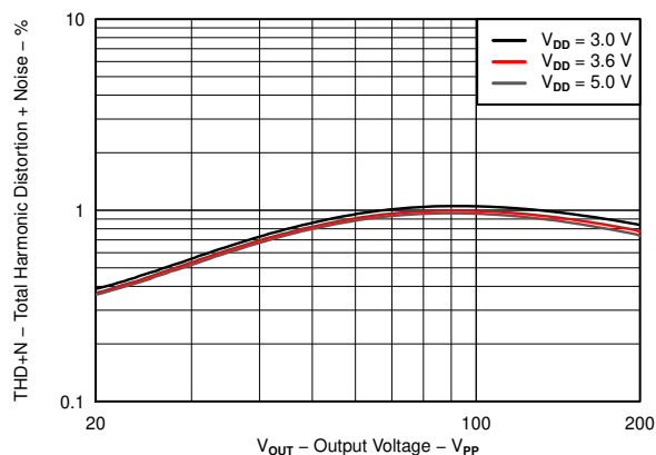
FIG 6-9. Total Harmonic Distortion + Noise vs Output Voltage
