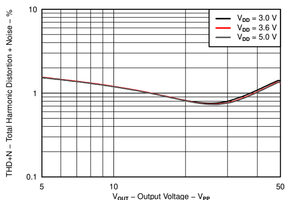
FIG 6-11. Total Harmonic Distortion + Noise vs Output Voltage
