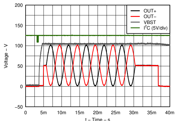
FIG 6-10. Typical Waveform
