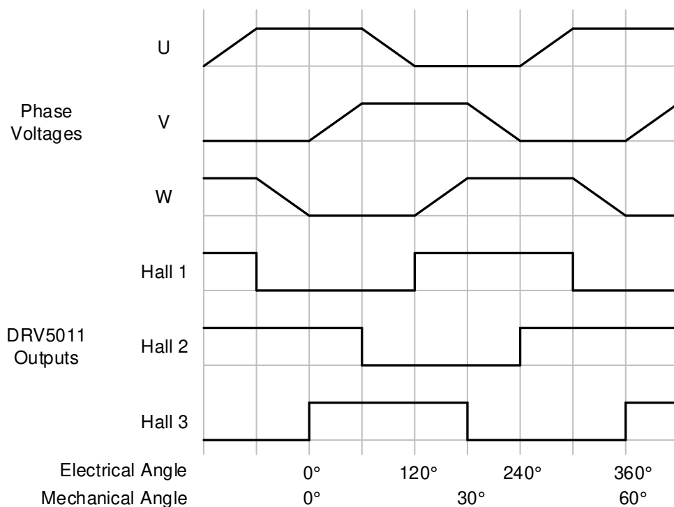
FIG 19. Phase Voltages and Hall Signals for a 3-Phase BLDC Motor
