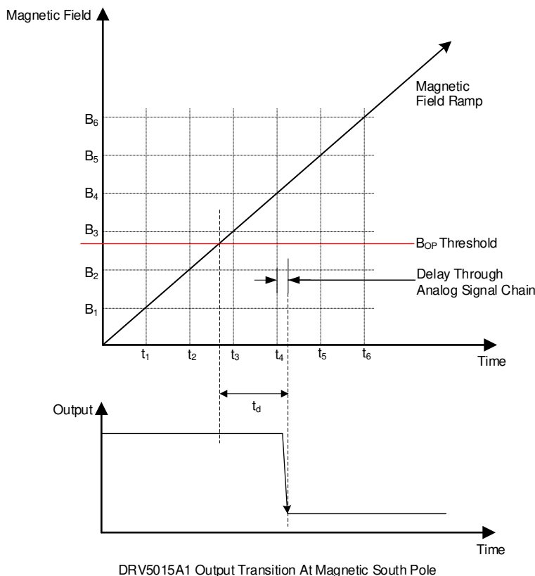
Figure 17. Propagation Delay
