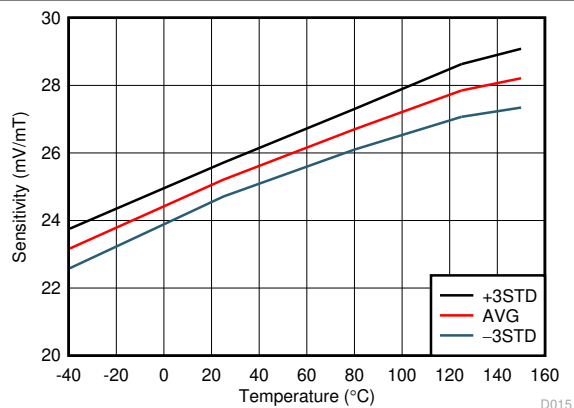
图 5-13. Sensitivity vs Temperature
