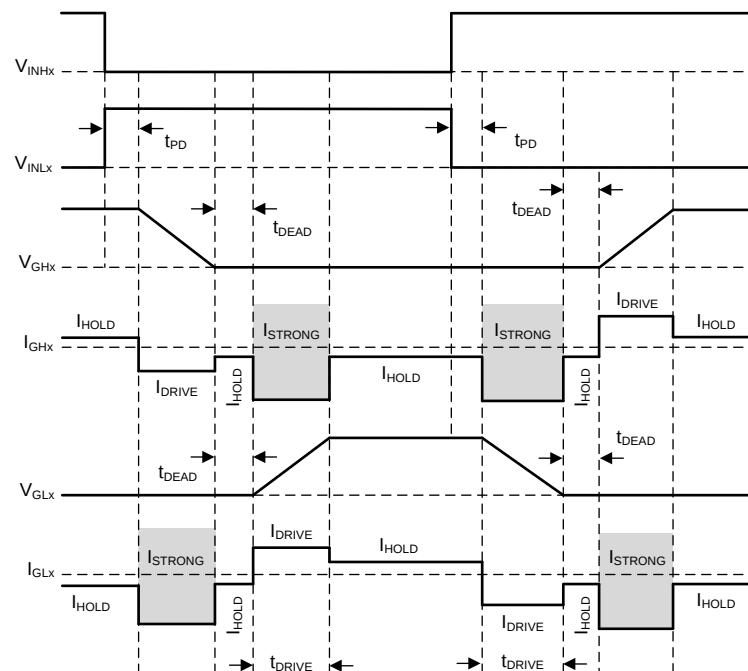
☒ 21. TDRIVE State Machine
