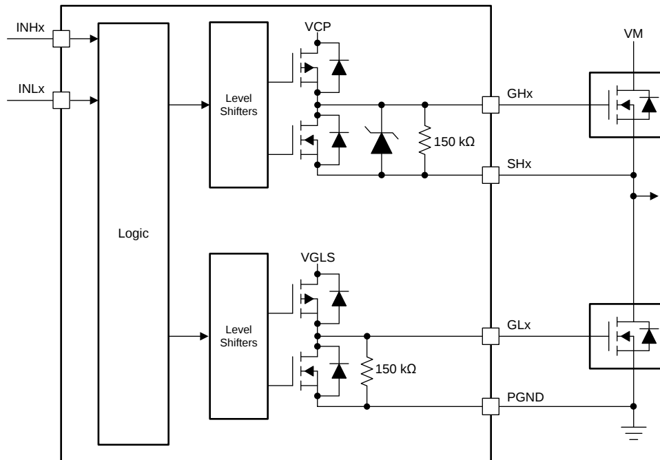
FIG 20. Gate Driver Block Diagram
