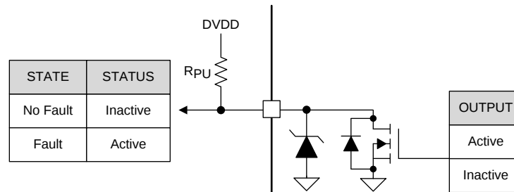
Figure 29. Open-Drain Output Pin Structure
