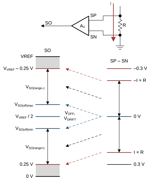
FIG 46. Sense Amplifier Configuration
