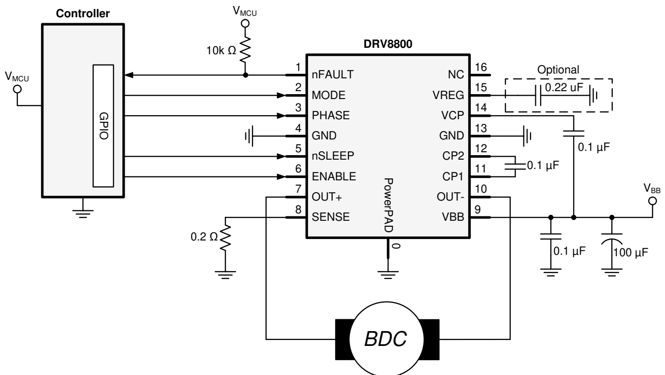
9-1. DRV8800 Typical Application Schematic
