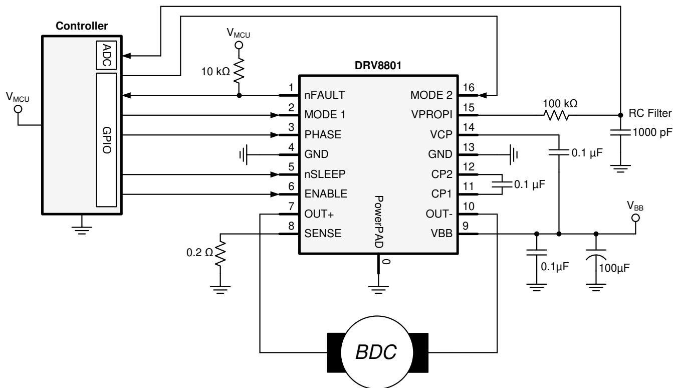
9-2. DRV8801 Typical Application Schematic
