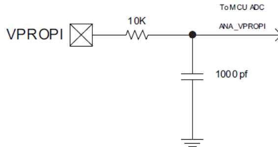
図 7-3. RC Network in Series With the VPROPI Output
