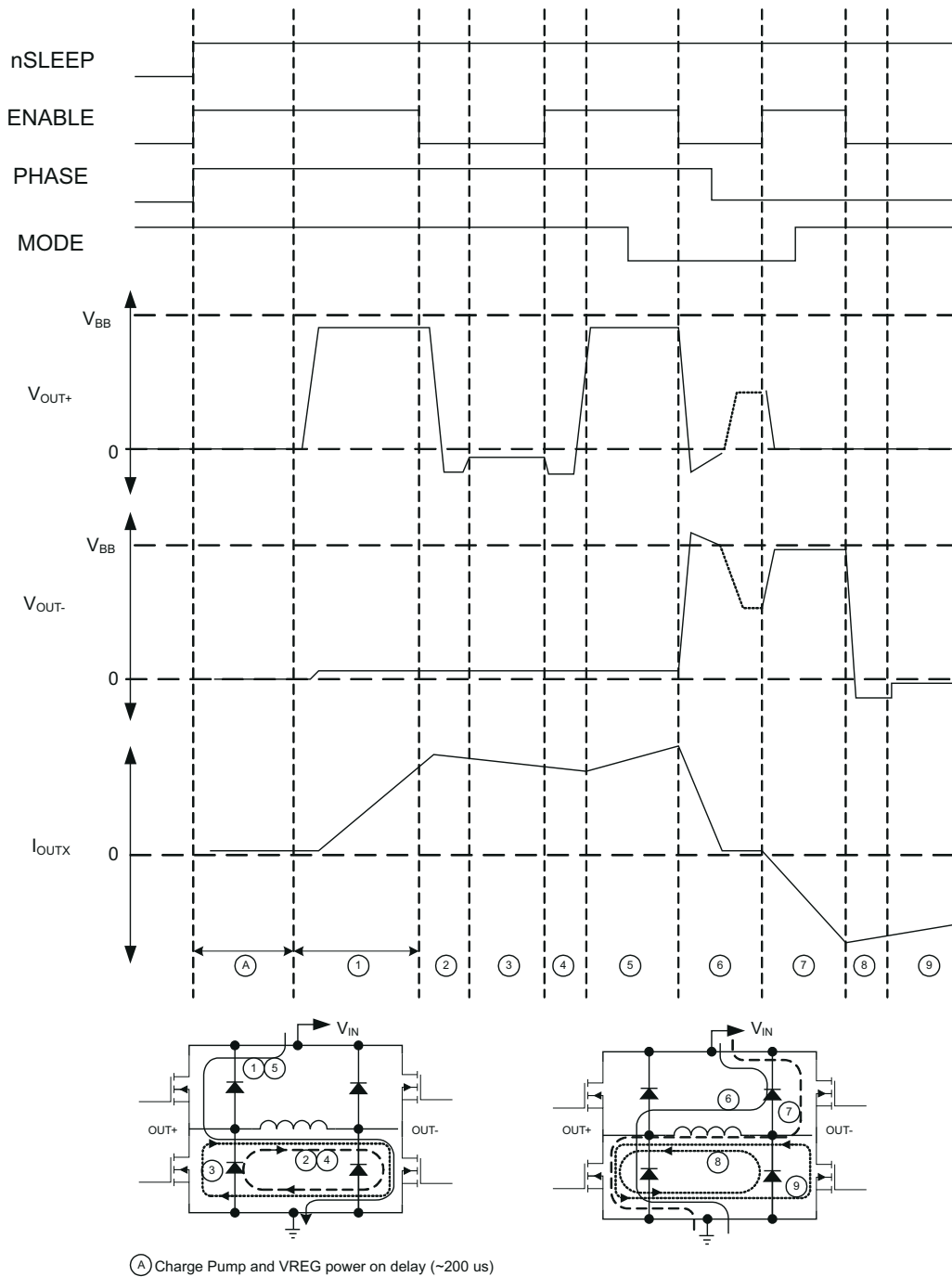
6-1. PWM Control Timing
