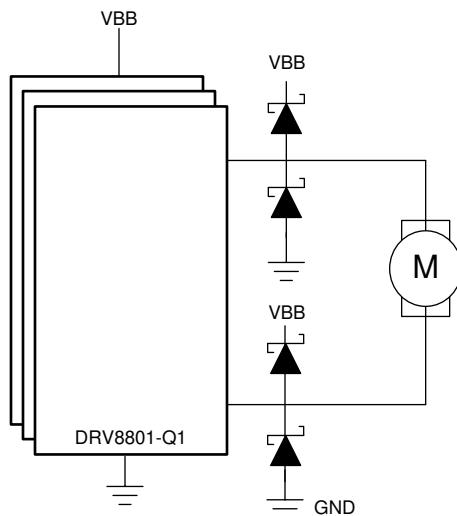
8-9. Schottky Diodes Connection
