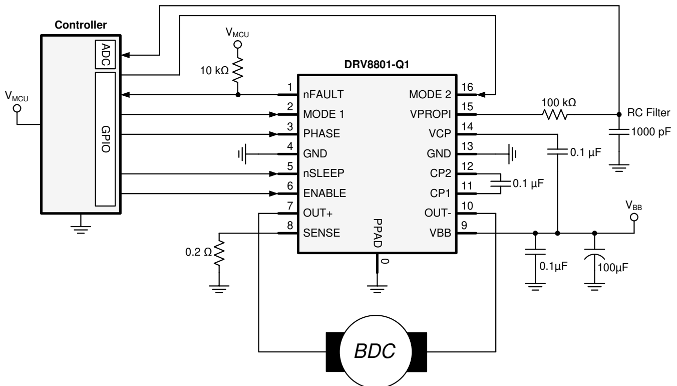
8-1. Typical Application Schematic
