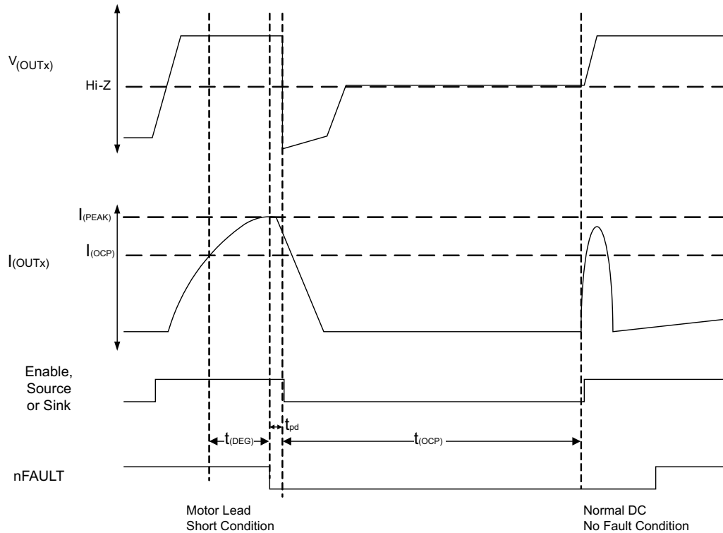
FIG 7-2. Overcurrent Control Timing
