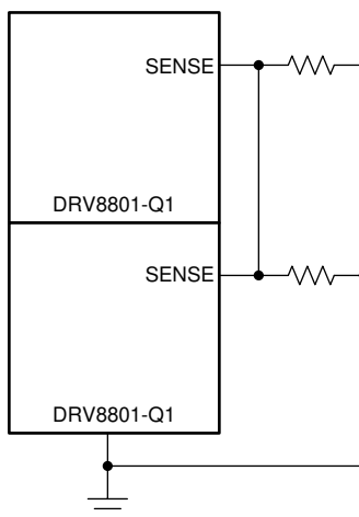
8-10. SENSE Resistors Connection
