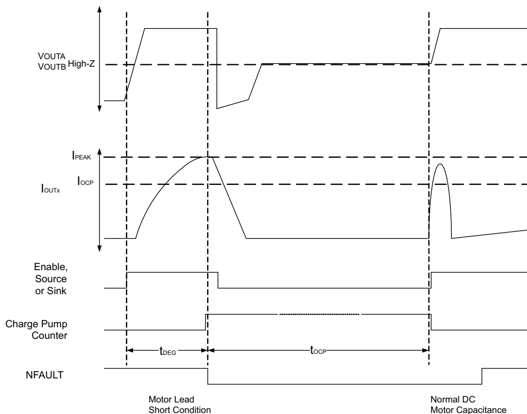
6-2. Overcurrent Control Timing
