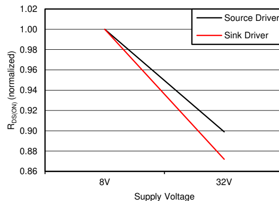
Figure 6-4. R_{DS(ON)} vs V_{BB} (Normalized to V_{BB} = 8\text{ V} )
