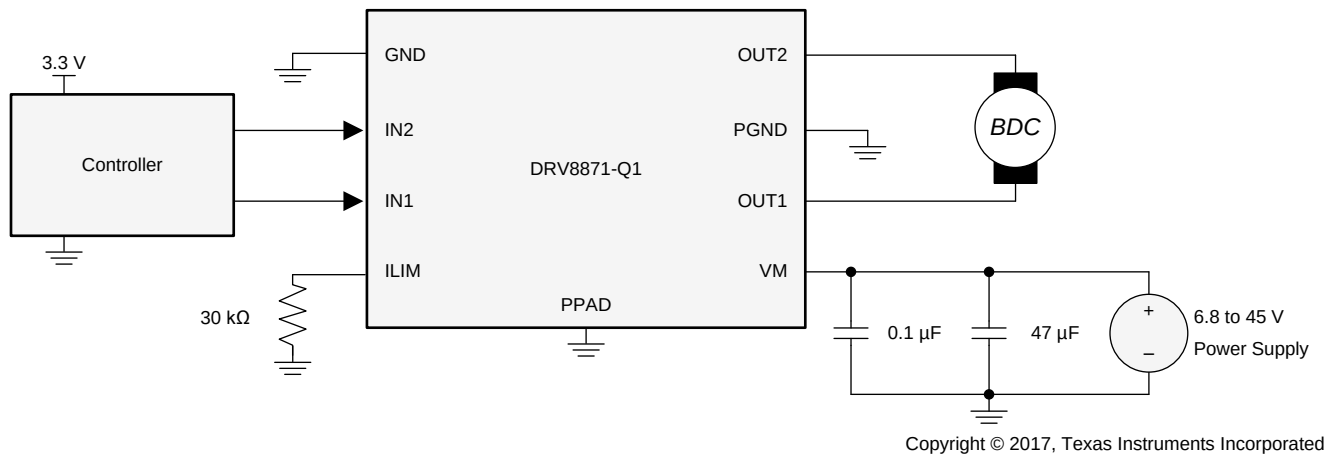
図 7. Typical Connections
