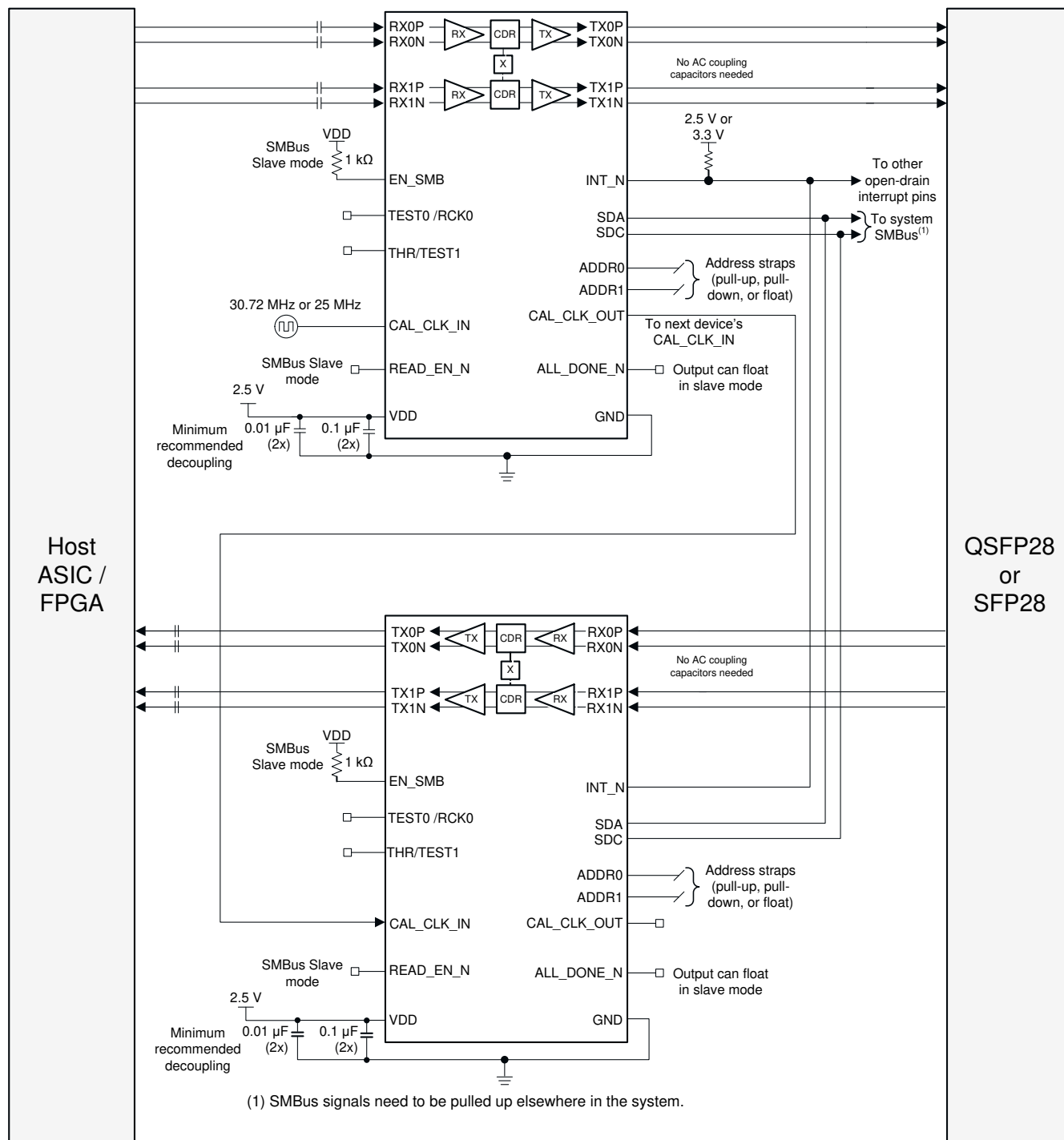
9-4. Front-Port Application Schematic
