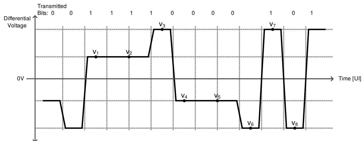
Figure 8-3. Conceptual FIR Waveform With Pre-Cursor Only
