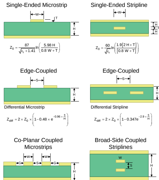
Figure 19. Controlled-Impedance Transmission Lines
