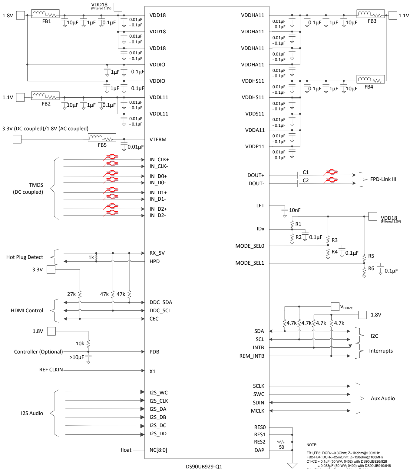
Figure 22. Typical Application Connection -- STP
