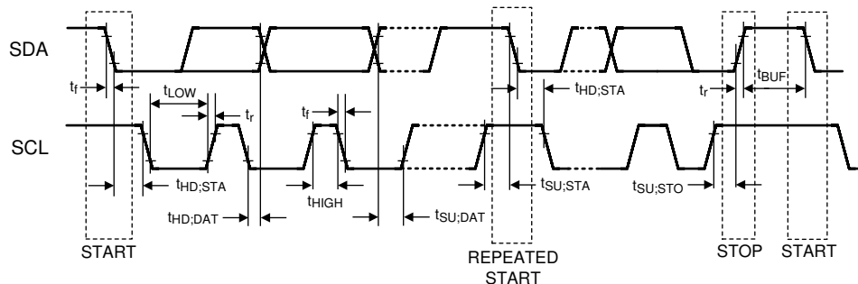
FIG 4-4. I2C Serial Control Bus Timing
