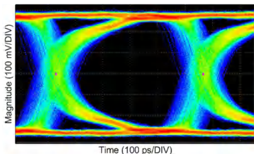
図 6-7. CMLOUTP/N Loop-through Eye Diagram at 1.867 Gbps 15 Meters of DACAR 462 Cable
