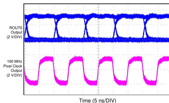
図 6-8. ROUT0 Data Sampled by 100-MHz PCLK RRFB (0x3B[0]) = 1
