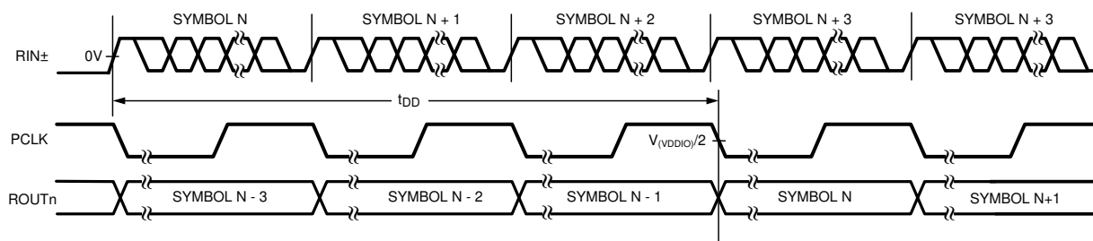
FIG 4-6. Deserializer Delay
