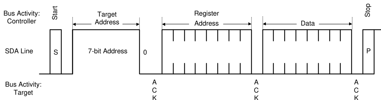
5-9. Serial Control Bus — WRITE
