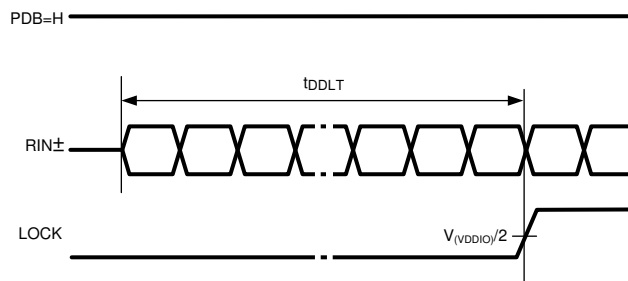
4-3. Deserializer Data Lock Time
