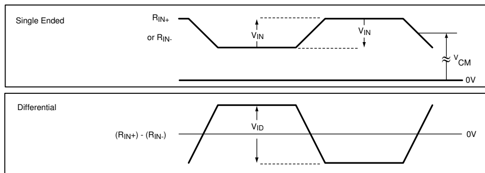
4-2. FPD-Link III Receiver V_{ID} , V_{IN} , V_{CM}
