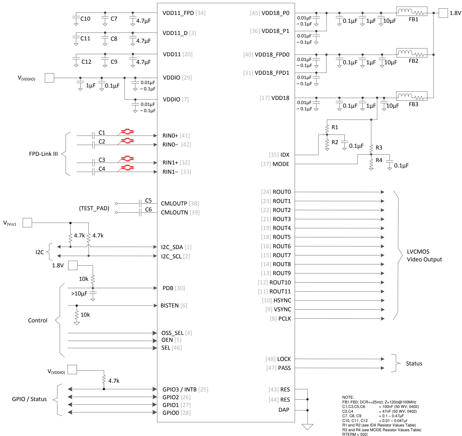
6-4. Typical Connection Diagram STP
