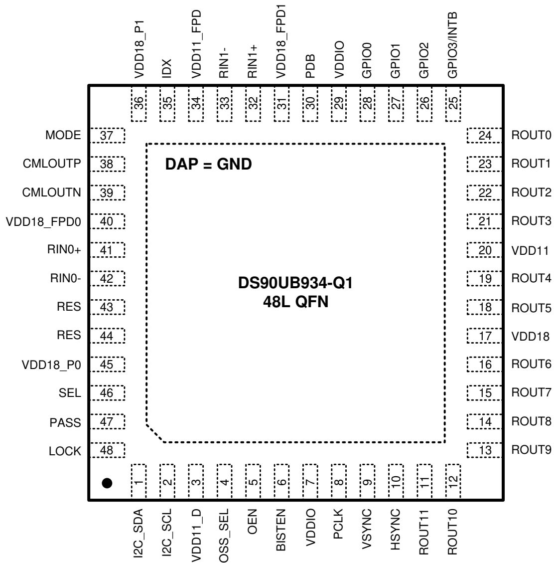
FIG 4-1. RGZ Package 48-Pin VQFN With Thermal Pad Top View
