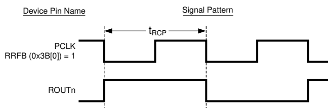
FIG 4-5. SSO Test Pattern for Power Consumption
