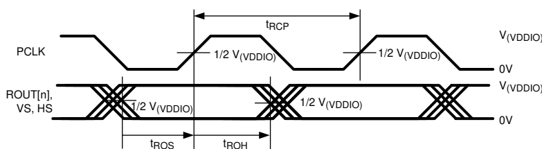
FIG 4-7. Deserializer Output Setup/Hold Times
