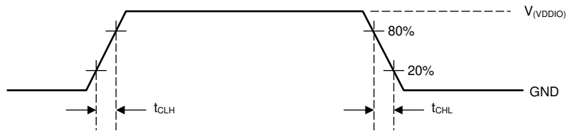
6-1. LVCMOS Transition Times
