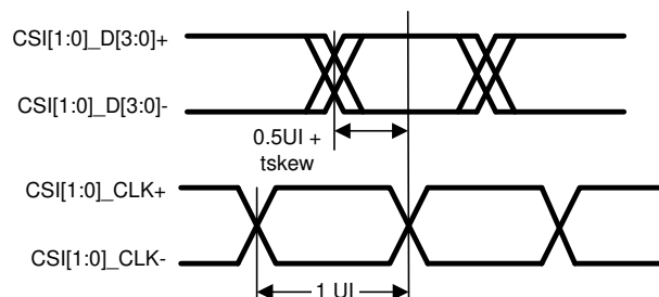
FIG 10. Clock and Data Timing in HS Transmission
