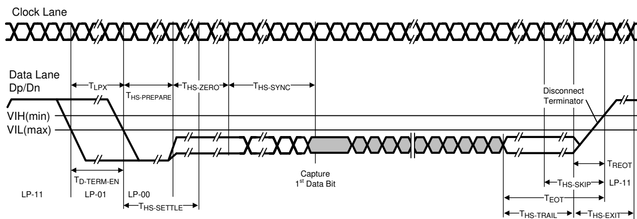
FIG 11. High-Speed Data Transmission Burst
