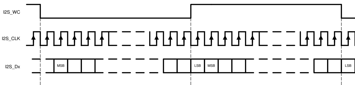
☒ 7-8. I2S Frame Timing Diagram
