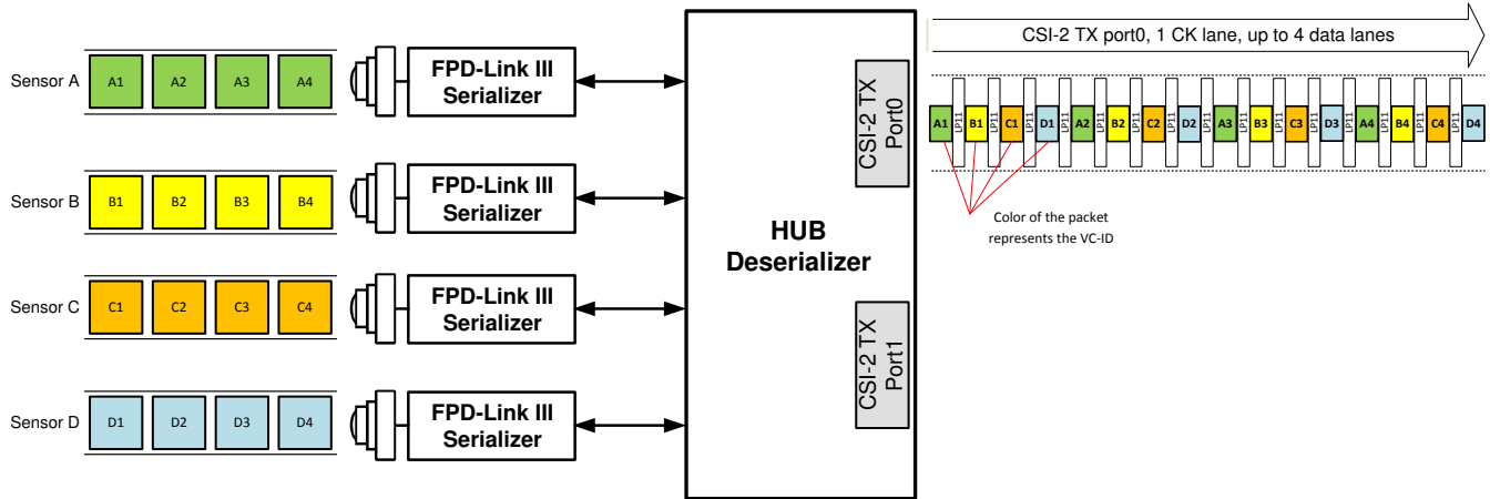
図 7-13. Four Sensor Data onto CSI-2 With Virtual Channels (VC-ID)
