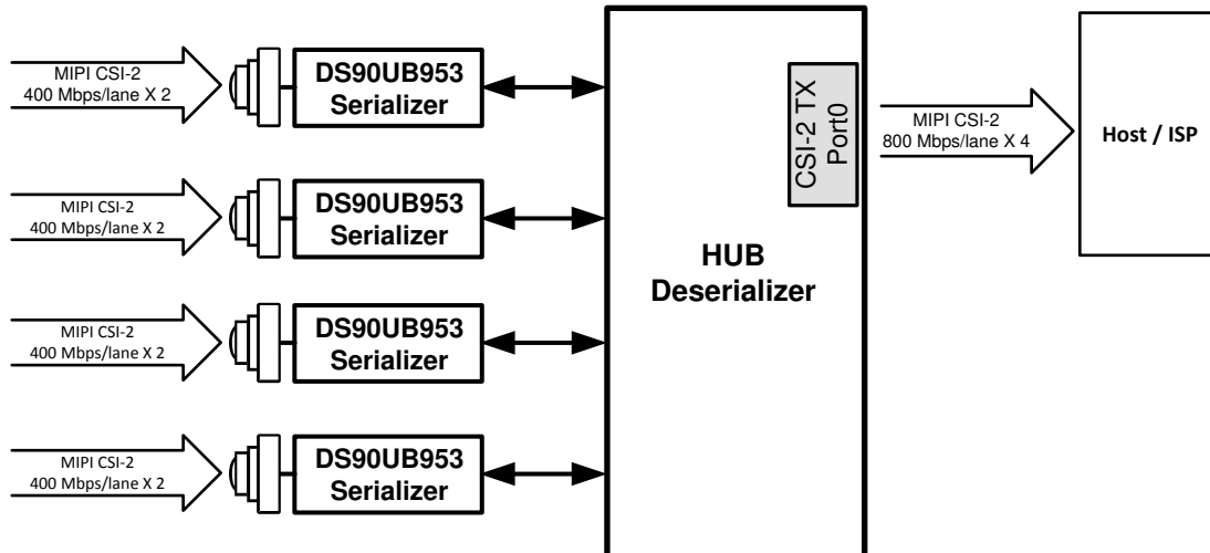
8-13. Four DS90UB953-Q1 Sensor Data Onto CSI-2 Over 1 Port
