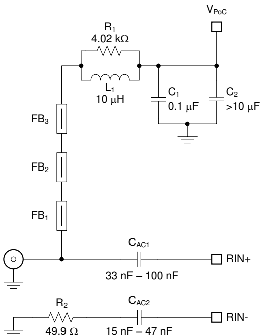
8-2. Example Recommended PoC Network for a "4G" FPD-Link III
