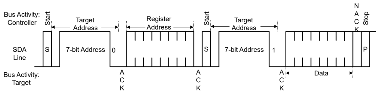
図 7-24. Serial Control Bus — READ
