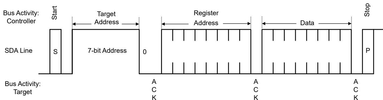
図 7-25. Serial Control Bus — WRITE
