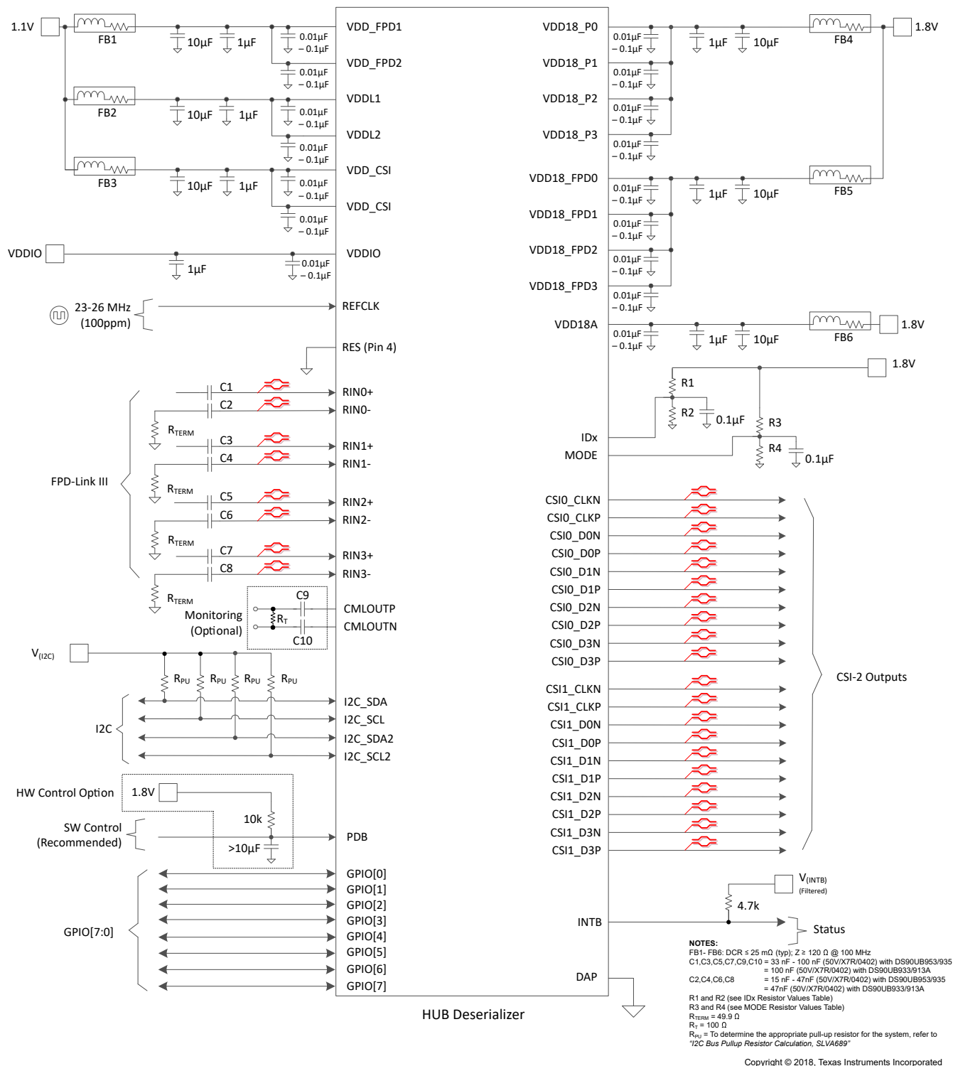
図 8-4. Typical Connection Diagram (Coaxial)
