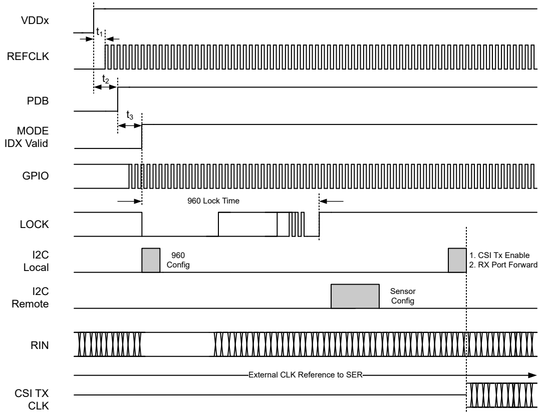
8-20. Power-Up Sequencing With Non-synchronous Clocking Mode
