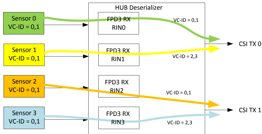
図 7-12. VC-ID Mapping Example 2
