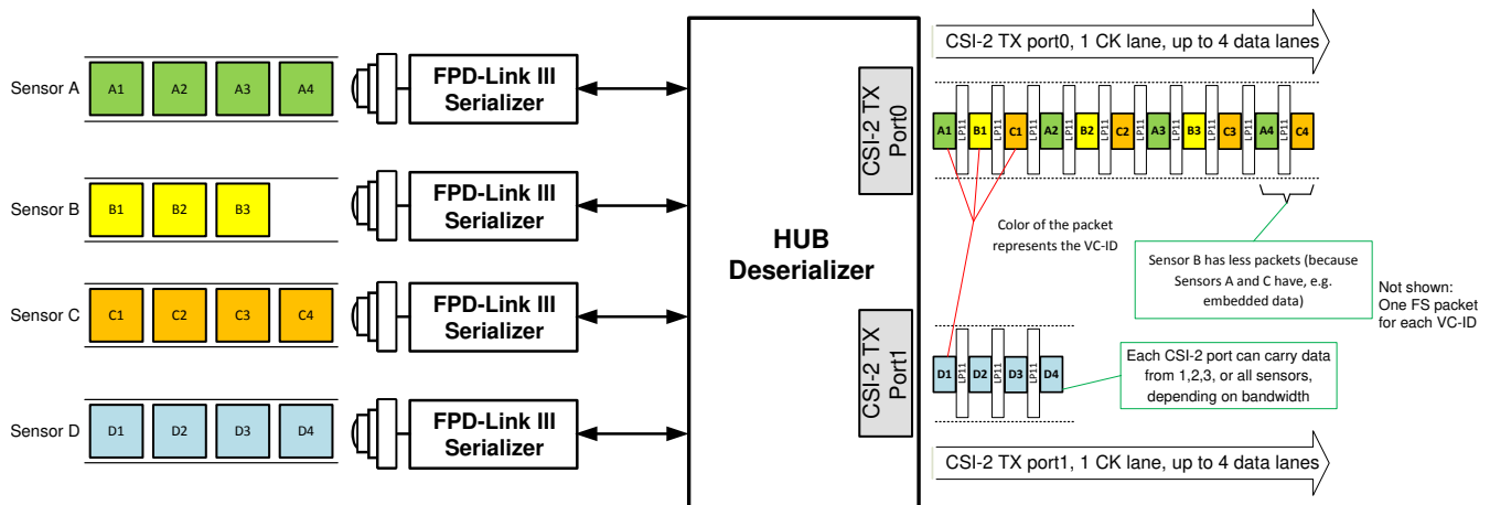
図 7-14. Four Sensor Data onto CSI-2 With Virtual Channels (VC-ID) With Different Frame Size
