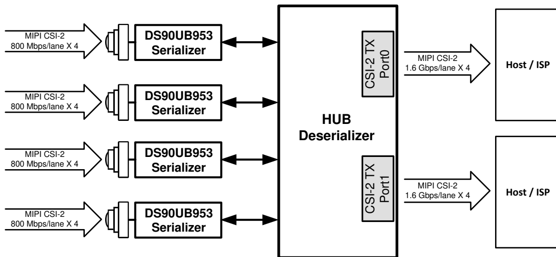
8-12. Four DS90UB953-Q1 Sensor Data Onto CSI-2 Over 2 Ports
