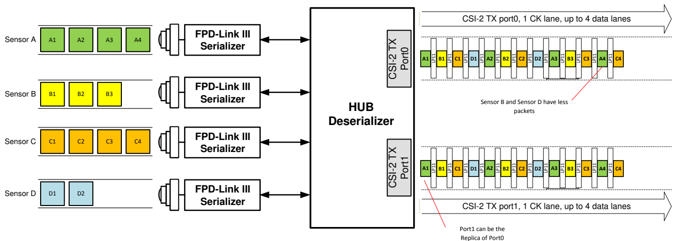
図 7-15. Four Sensor Data onto 1xCSI-2 Replicated With Virtual Channels (VC-ID) With Different Frame Size
