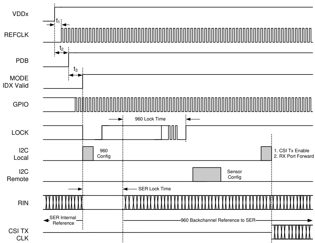
8-19. Power-Up Sequencing With Synchronous Clocking Mode
