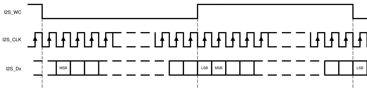
図 7-8. I2S Frame Timing Diagram
