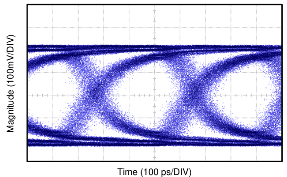
图 8-6. Loop-Through CML Output at 2.6-Gbps Serial Line Rate
