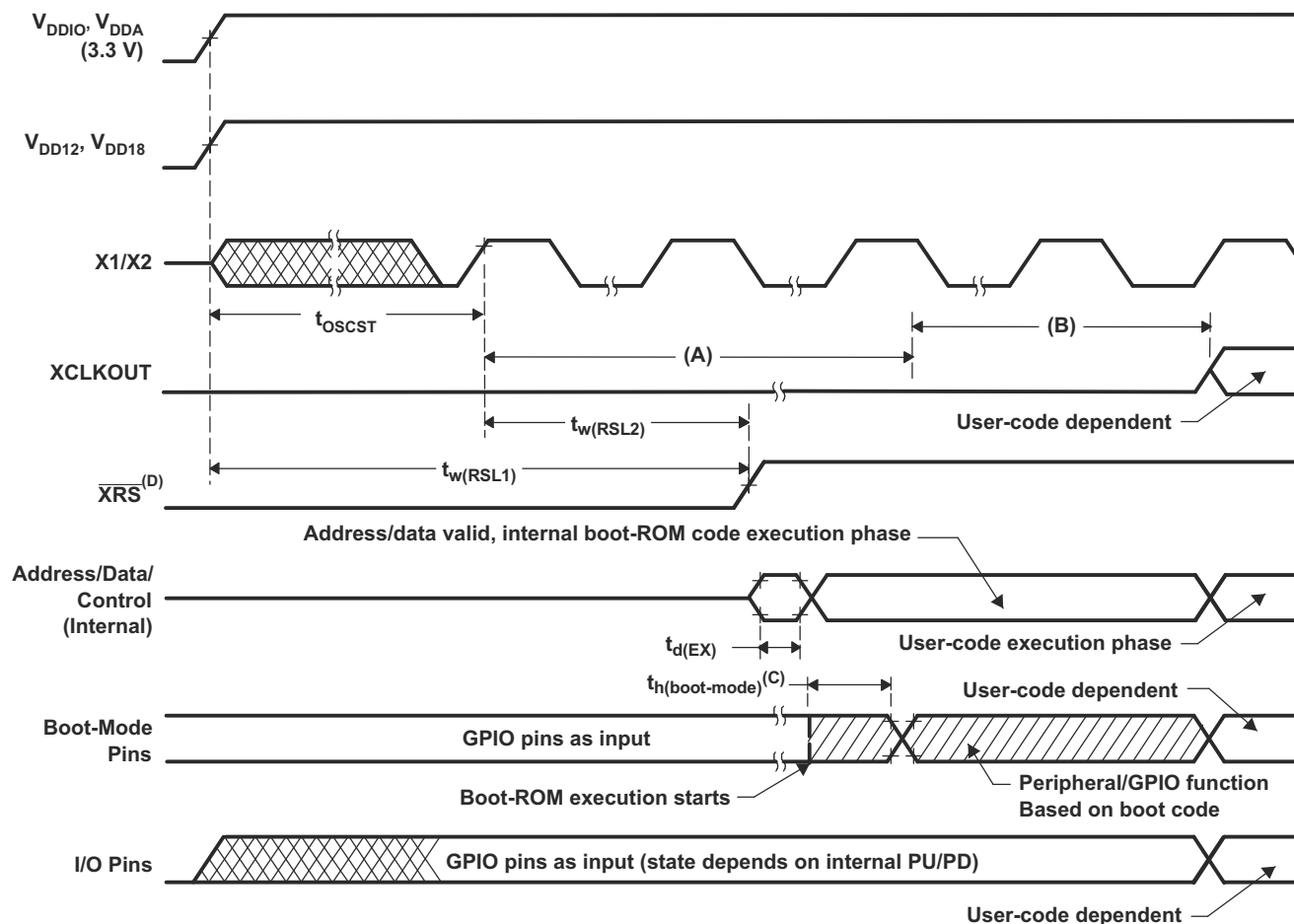
FIG 7-1. Power-On Reset
