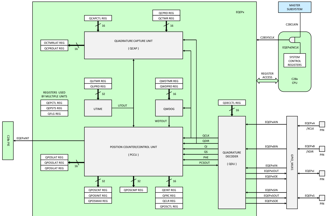
7-47. eQEP
