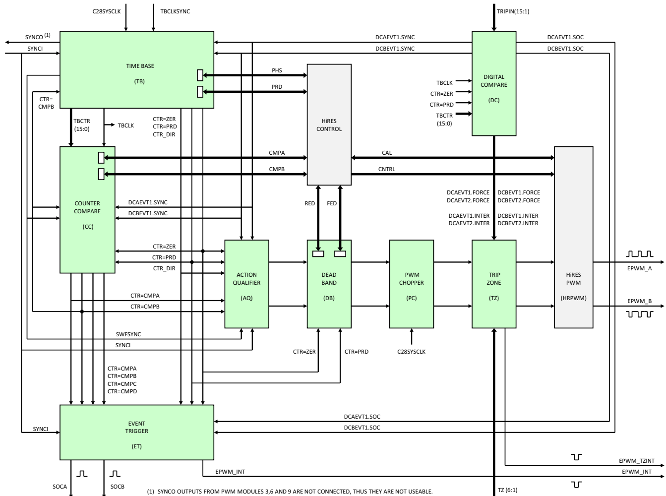
7-44. Internal Structure of PWM
