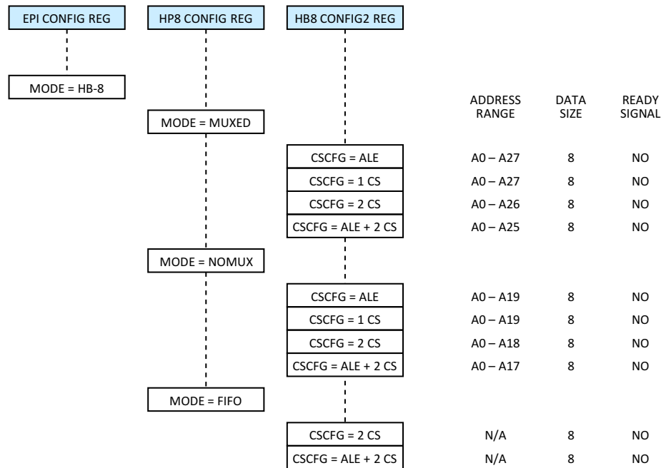
図 7-19. EPI 8-Bit Host Bus Mode
