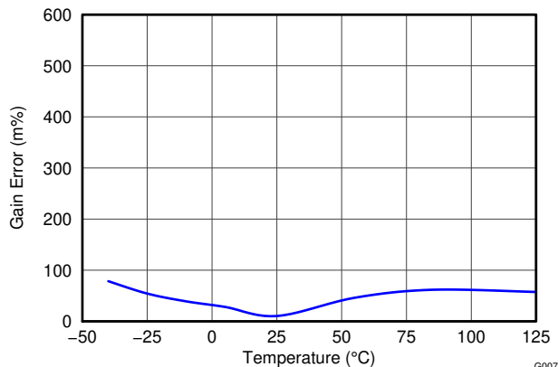
FIG 5-6. Shunt Input Gain Error vs Temperature
