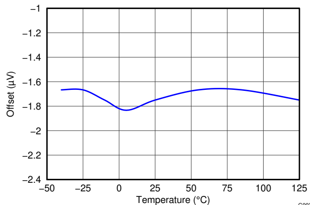
FIG 5-3. Shunt Input Offset Voltage vs Temperature
