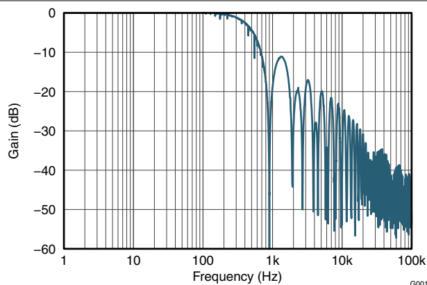
FIG 5-1. Frequency Response
