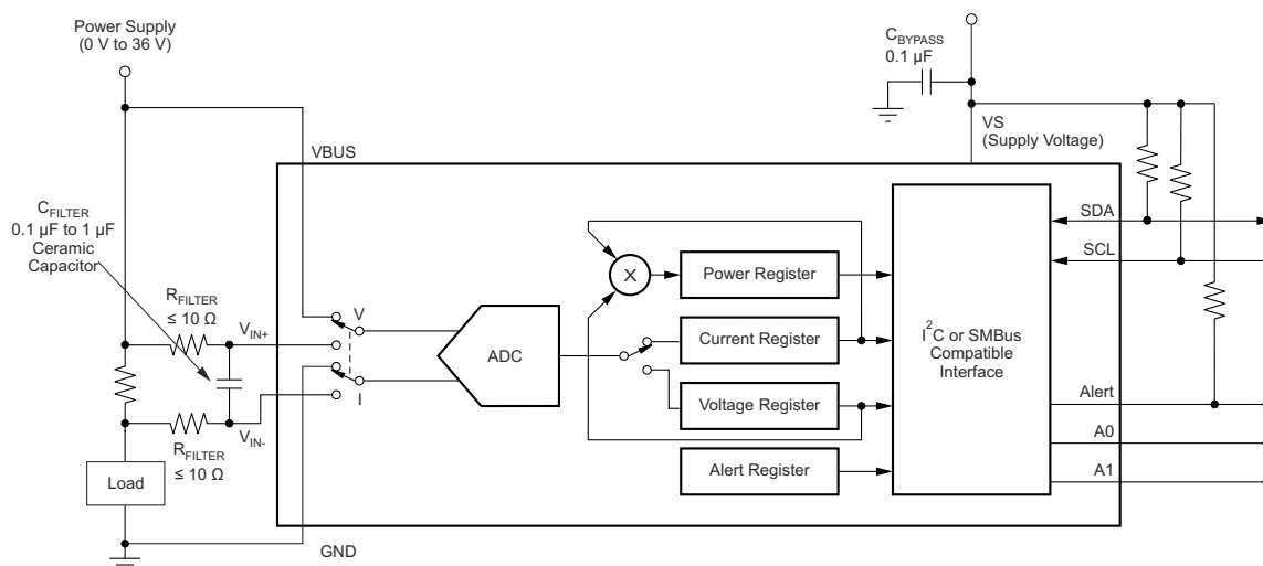
☒ 6-3. Input Filtering
