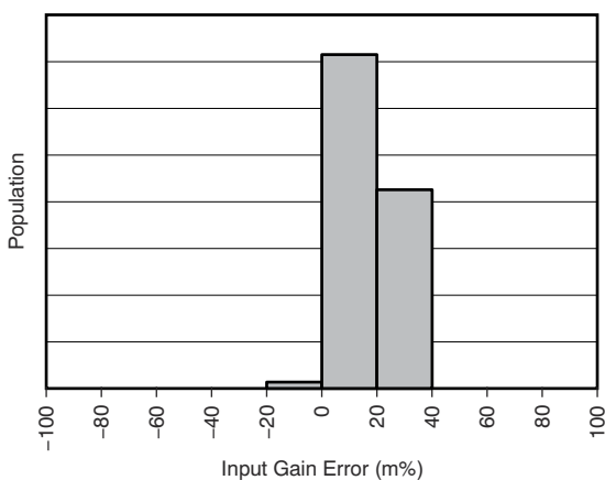
FIG 5-5. Shunt Input Gain Error Production Distribution
