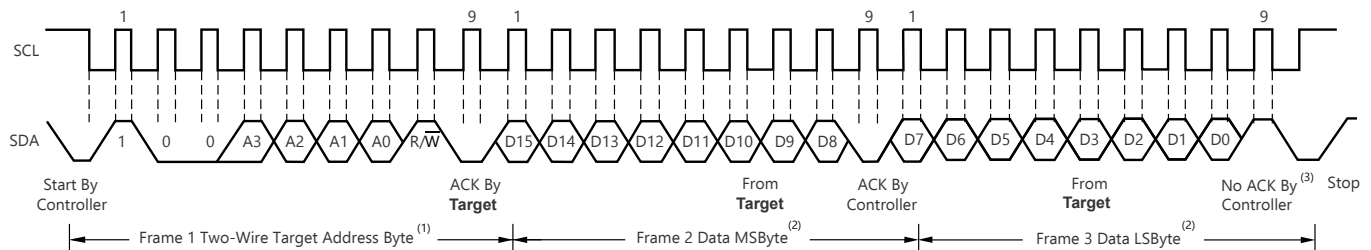
図 6-4. Timing Diagram for Write Word Format
