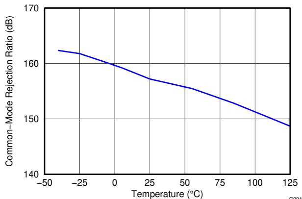
FIG 5-4. Shunt Input Common-Mode Rejection Ratio vs Temperature
