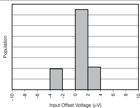
FIG 5-2. Shunt Input Offset Voltage Production Distribution
