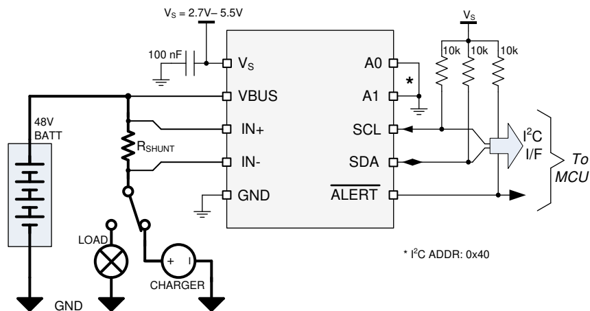
8-2. INA238-Q1 High-Side Sensing Application Diagram
