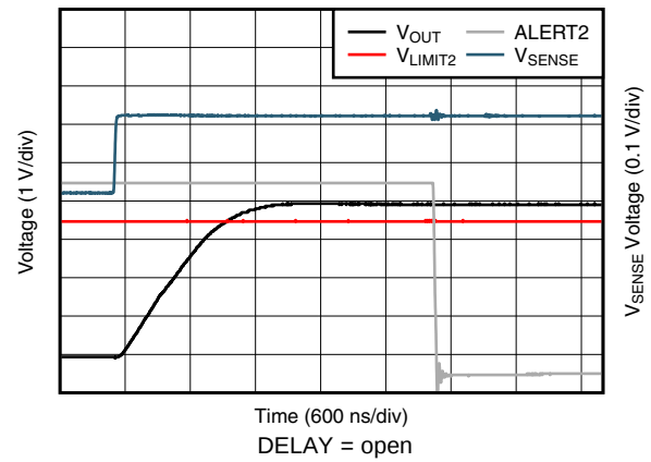
FIG 32. Comparator 2 Total Propagation Delay (INA303)
