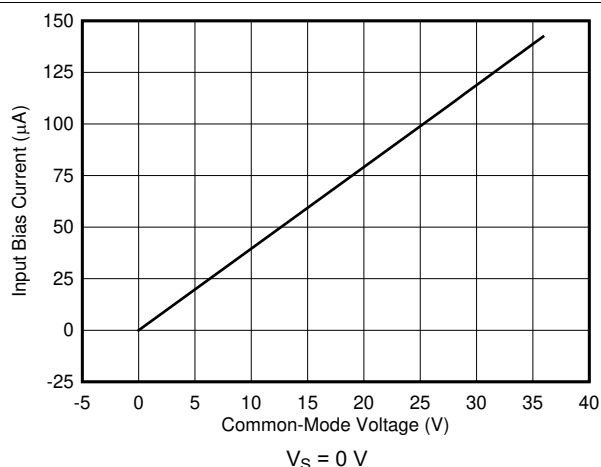
FIG 6-18. Input Bias Current vs. Common-Mode Voltage
