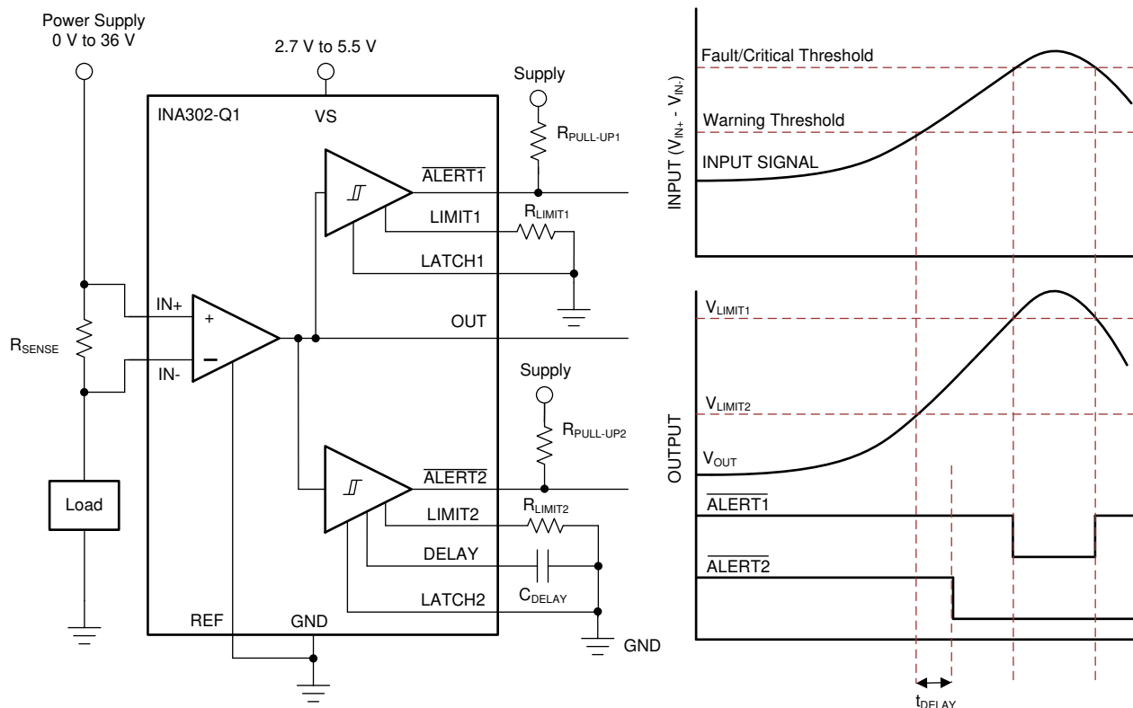
7-1. Out-of-Range Alert Responses for the INA302-Q1
