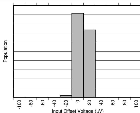
FIG 6-2. Input Offset Voltage Distribution (INA30xA2-Q1)
