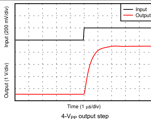
FIG 6-24. Voltage Output Rising Step Response
