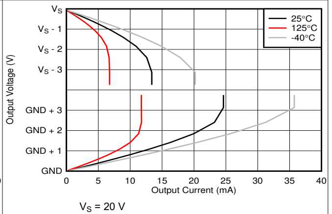
6-20. Output Voltage vs Output Current
