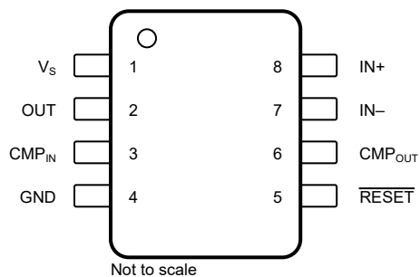
図 5-1. INA310x-Q1: DGK Package 8-Pin VSSOP Top View
