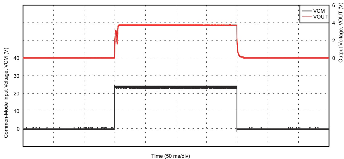
8-2. Solenoid Control Current Response
