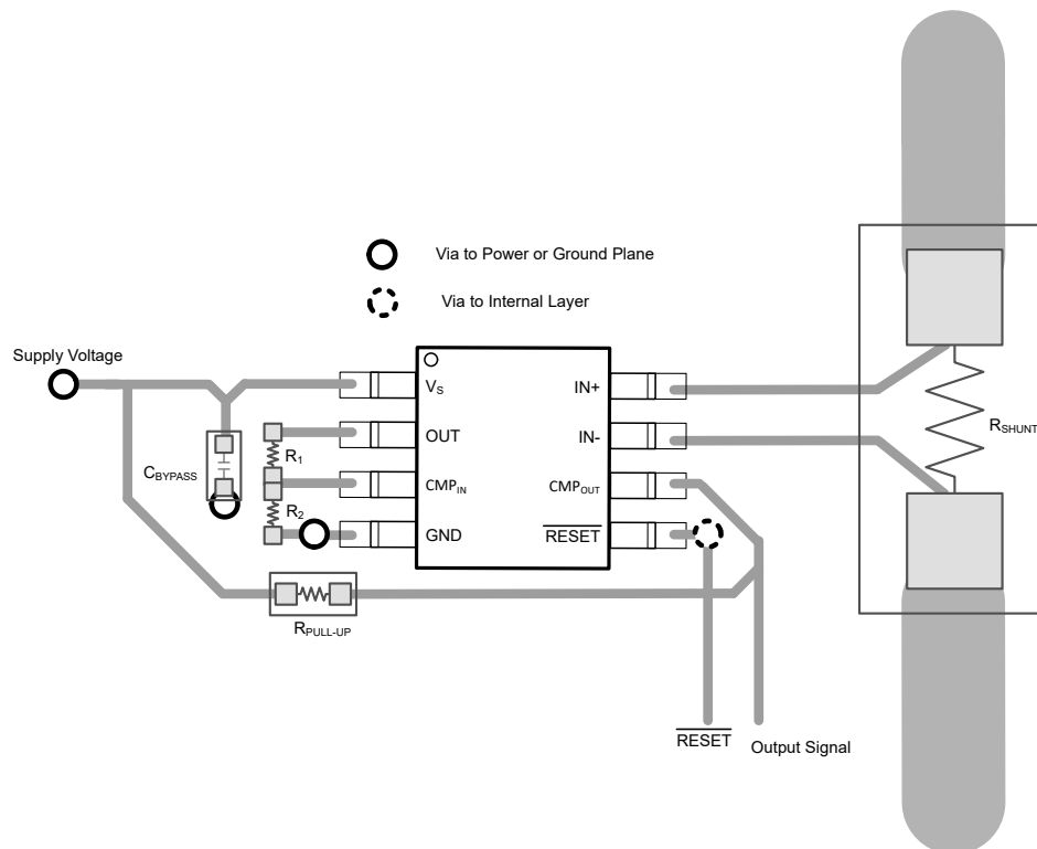
8-5. INA310x-Q1 Recommended Layout
