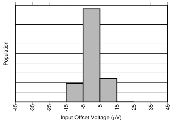
FIG 6-3. INA310A3-Q1 Input Offset Production Distribution
