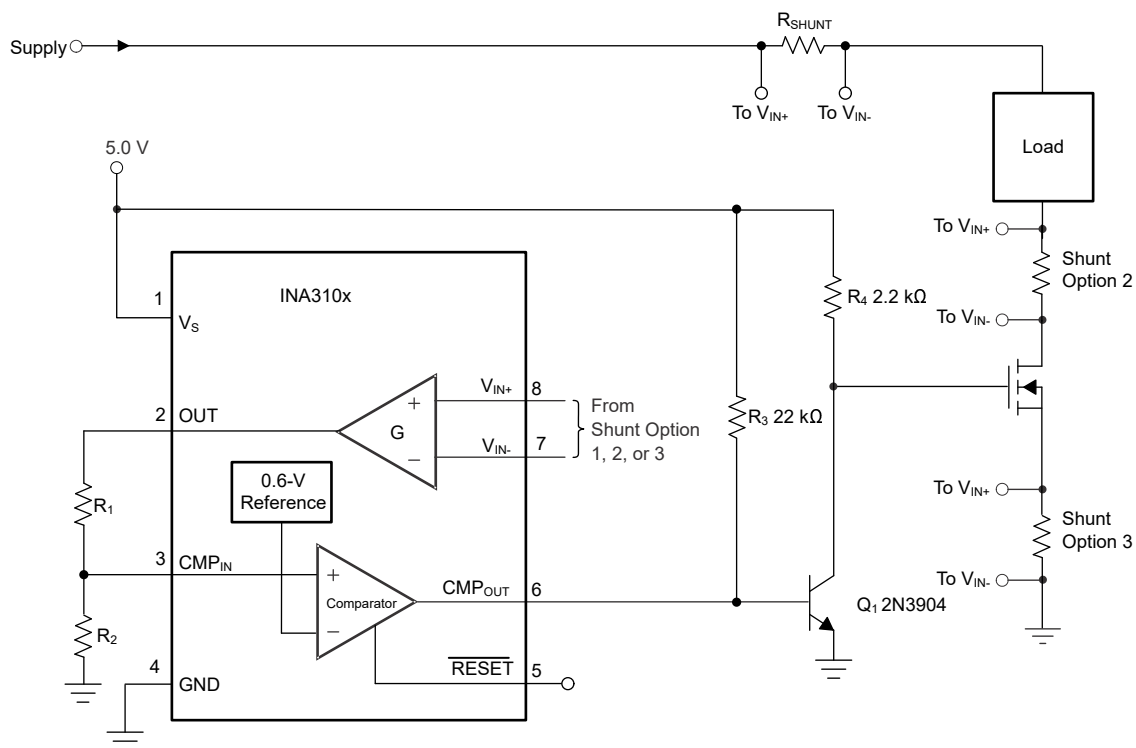
8-3. Low-Side Switch Overcurrent Shutdown
