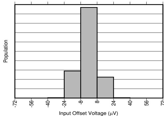
FIG 6-2. INA310A2-Q1 Input Offset Production Distribution
