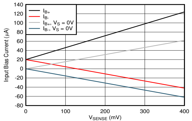
6-16. INA310x2-Q1, INA310x3-Q1 Input Bias Current vs V_{SENSE}
