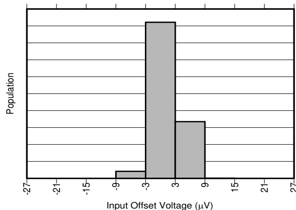
FIG 6-4. INA310A4-Q1 Input Offset Production Distribution
