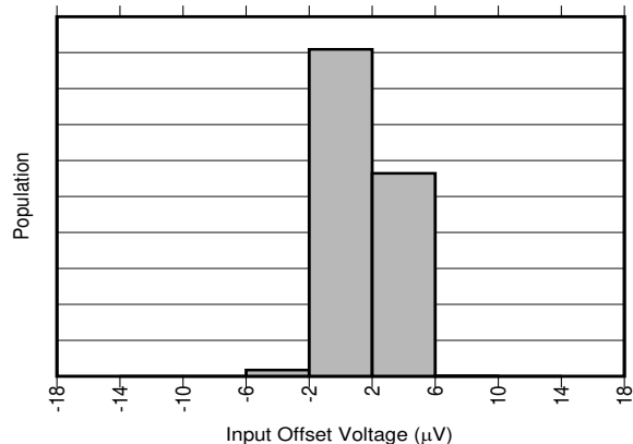
FIG 6-5. INA310A5-Q1 Input Offset Production Distribution
