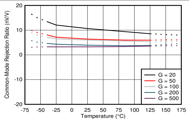
FIG 6-8. Common-Mode Rejection Ratio vs. Temperature
