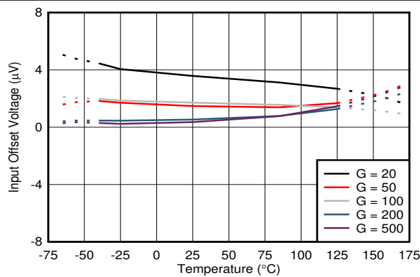
FIG 6-7. Input Offset Voltage vs. Temperature
