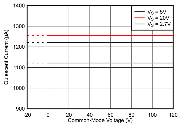
FIG 6-39. Quiescent Current vs. Common-Mode Voltage, INA4290
