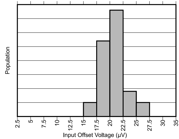
FIG 6-6. Input Offset Production Distribution, A1 Devices (INA4290)
