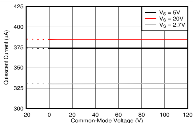
FIG 6-37. Quiescent Current vs. Common-Mode Voltage, INA290
