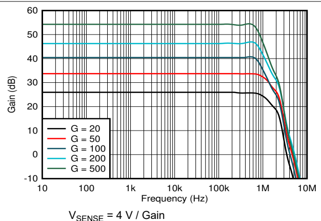
FIG 6-10. Gain vs. Frequency
