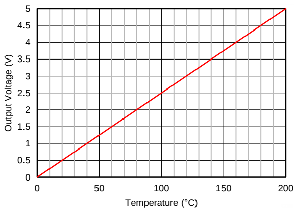
Figure 72. Transfer Function of 3-Wire RTD Interface
