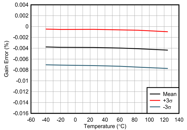
7-32. Gain Error vs Temperature
