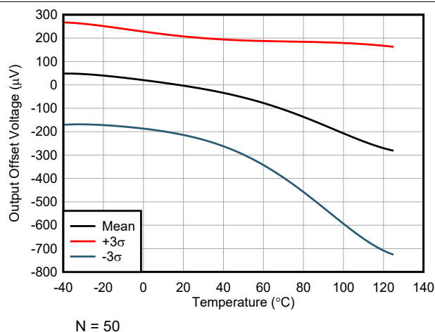
7-17. Input-Referred Output Offset Voltage vs Temperature
