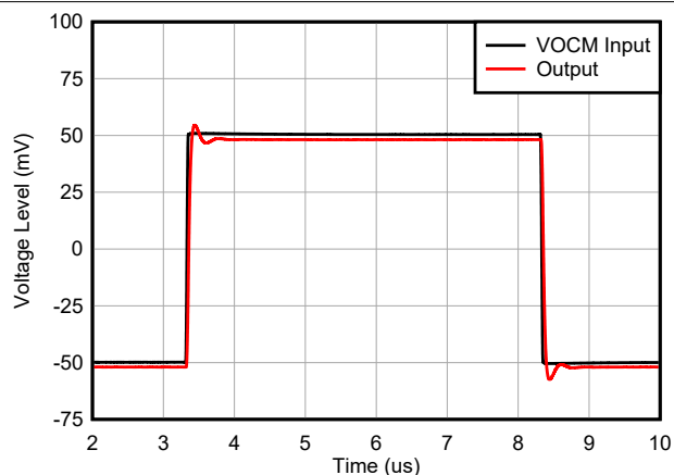
FIG 7-50. Small-Signal Response of VOCM Amplifier
