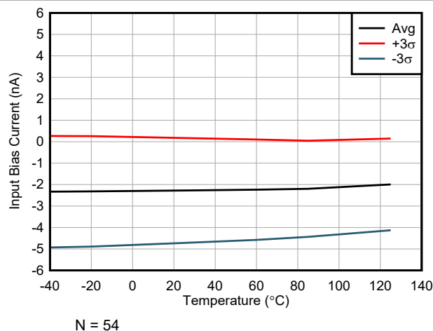
7-15. Input Bias Current vs Temperature
