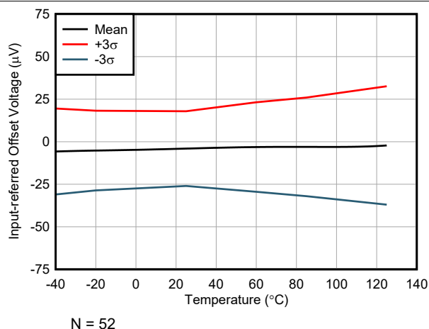
7-14. Input Stage Offset Voltage vs Temperature
