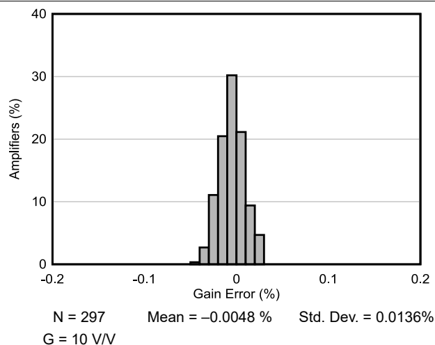
7-13. Typical Gain Error Distribution at G = 10 V/V
