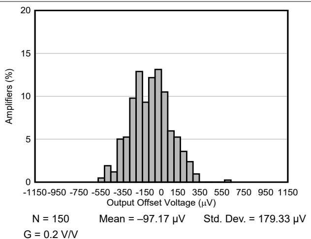
7-4. Typical Distribution of Output Offset Voltage
