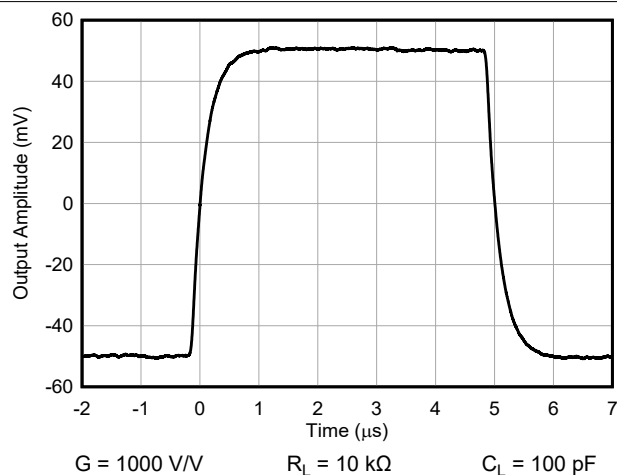
FIG 7-49. Small-Signal Response for G = 1000\text{ V/V}
