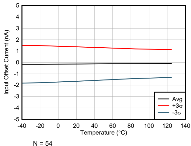
7-16. Input Offset Current vs Temperature
