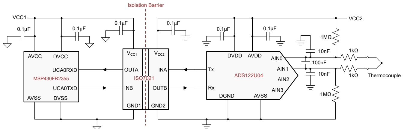
図 9-3. Isolated UART for a Temperature Field Transmitter
