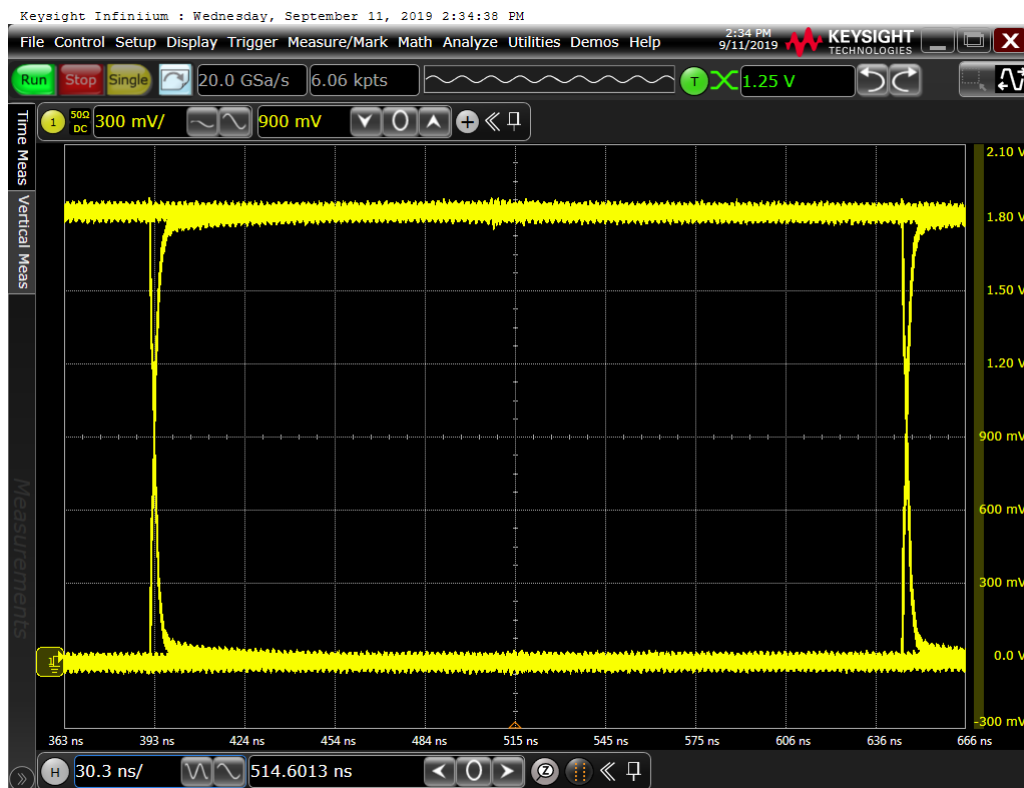
図 9-5. Eye Diagram at 4Mbps PRBS 2^{16} - 1 , 1.8V and 25°C
