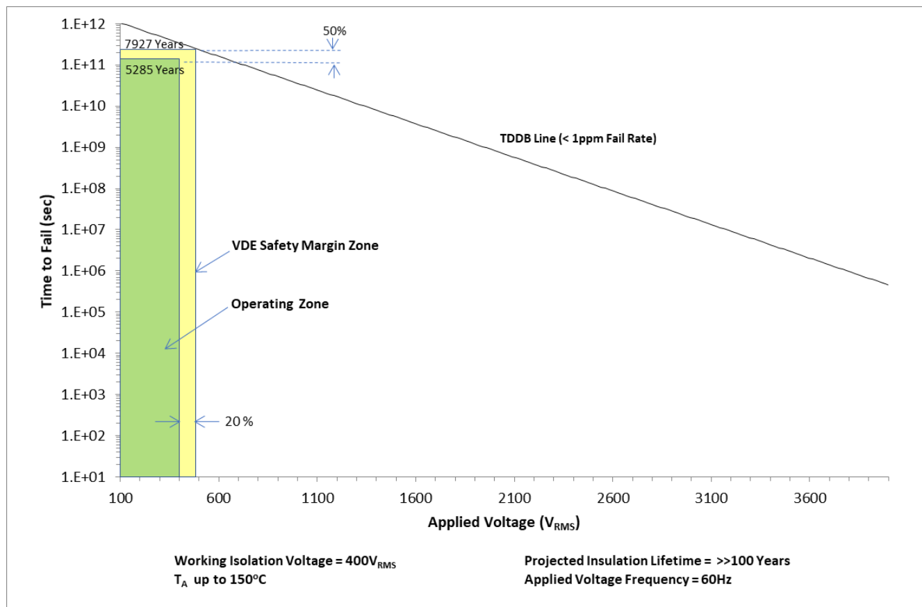
図 9-2. Insulation Lifetime Projection Data
