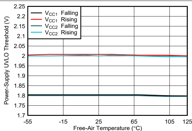
FIG 5-15. Power Supply Undervoltage Threshold vs Free-Air Temperature
