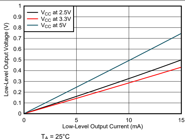
FIG 5-14. Low-Level Output Voltage vs Low-Level Output Current
