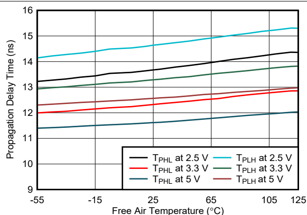
FIG 5-16. Propagation Delay Time vs Free-Air Temperature
