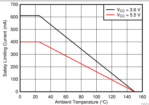
図 1. Thermal Derating Curve for Safety Limiting Current per VDE
