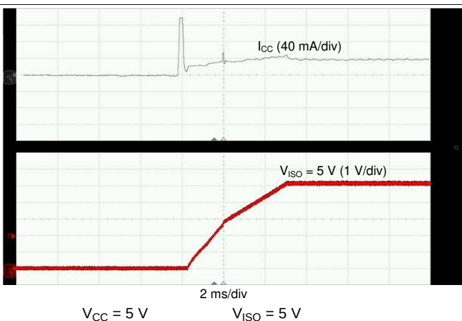
FIG 18. Soft Start at 10-mA Load
