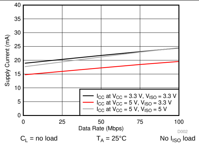
FIG 12. Supply Current vs Data Rate
