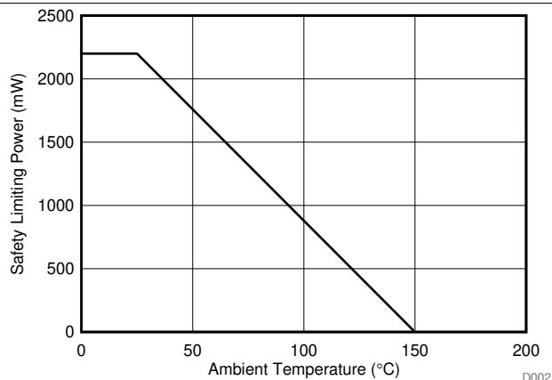
図 2. Thermal Derating Curve for Safety Limiting Power per VDE
