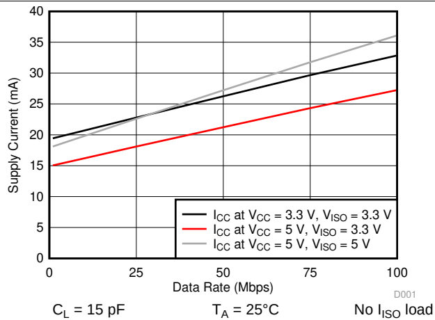
FIG 11. Supply Current vs Data Rate
