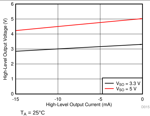
FIG 15. High-Level Output Voltage vs High-Level Output Current
