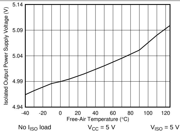
FIG 9. 5-V Isolated Supply Voltage ( V_{ISO} ) vs Free-Air Temperature
