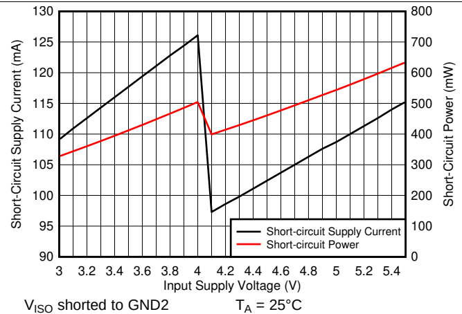
FIG 10. Short-Circuit Supply Current ( I_{CC} ) and Power (P) vs Supply Voltage ( V_{CC} )
