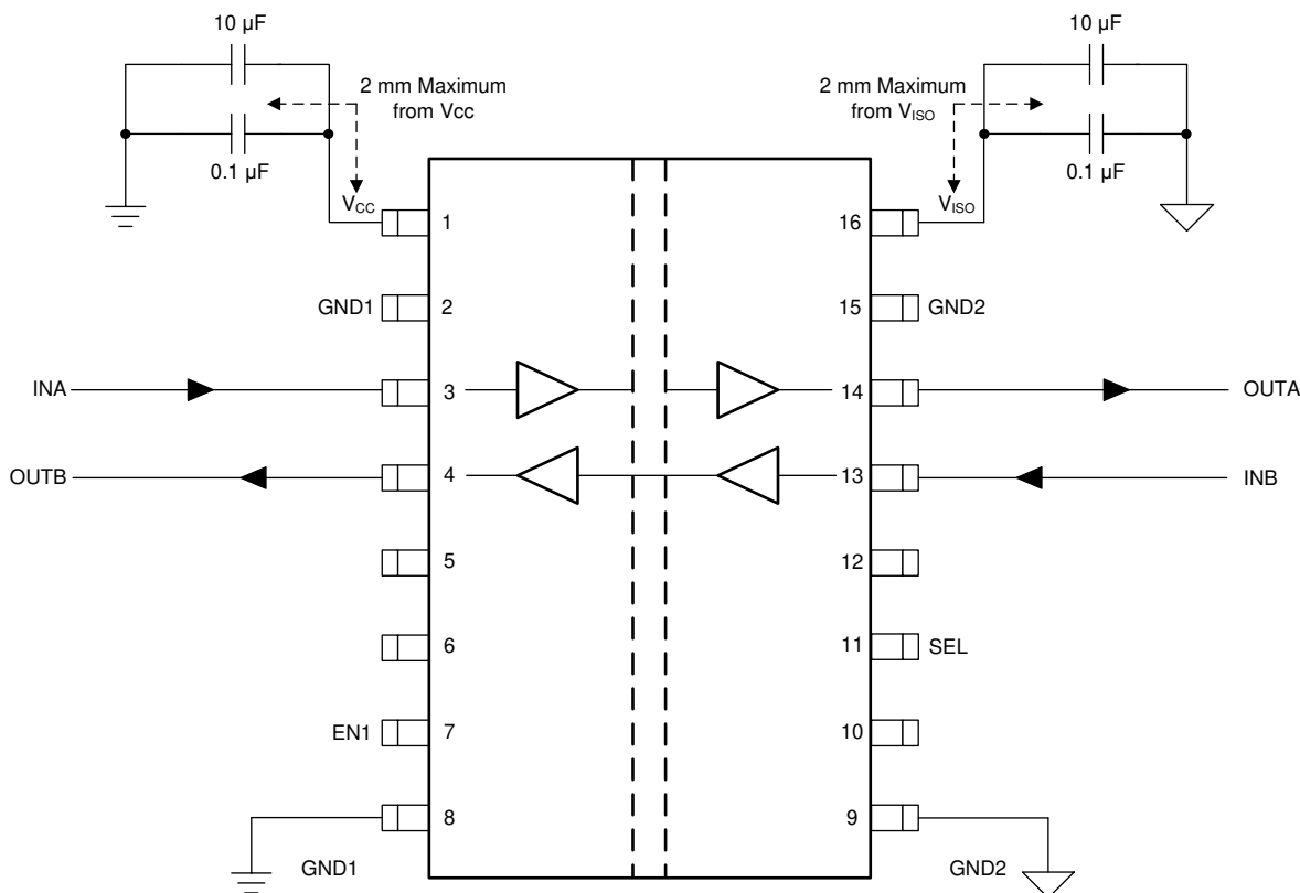
FIG 31. Typical Circuit Hook-Up
