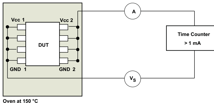
☒ 33. Test Setup for Insulation Lifetime Measurement
