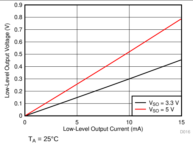
FIG 16. Low-Level Output Voltage vs Low-Level Output Current
