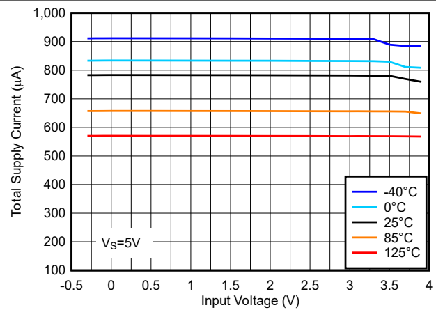
FIG 6-4. Total Supply Current vs. Input Voltage at 5V
