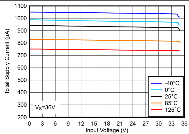
FIG 6-6. Total Supply Current vs. Input Voltage at 36V
