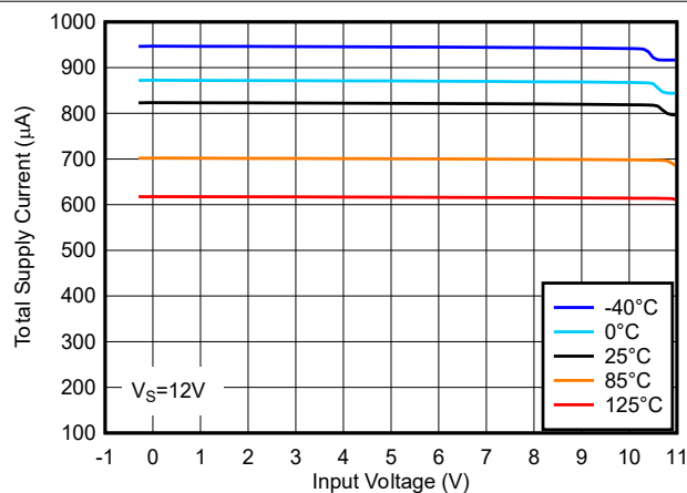
FIG 6-5. Total Supply Current vs. Input Voltage at 12V
