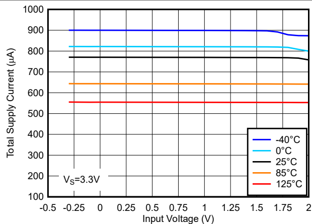
FIG 6-3. Total Supply Current vs. Input Voltage at 3.3V
