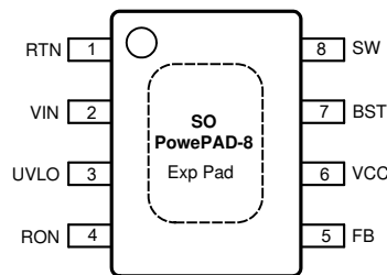
图 5-1. DDA Package Top View
