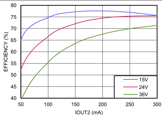
FIG 8-11. Efficiency at 500 kHz, V_{OUT1} = 5\text{ V}
