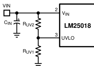
7-2. UVLO Resistor Setting
