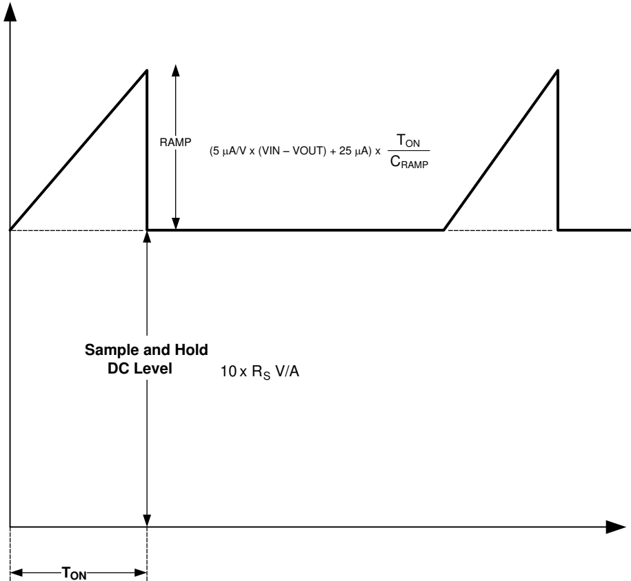
FIG 7-3. Composition of Current Sense Signal
