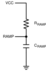
8-3. Additional Slope Compensation for V_{OUT} > 5\text{ V}
