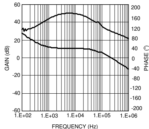
图 8-5. Error Amplifier Gain and Phase
