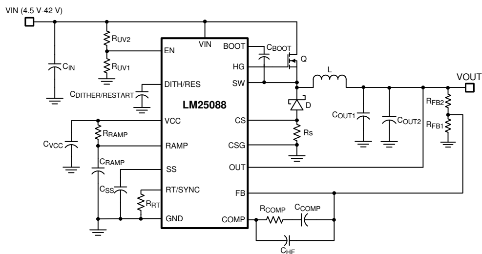
図 8-1. Simplified Application Schematic
