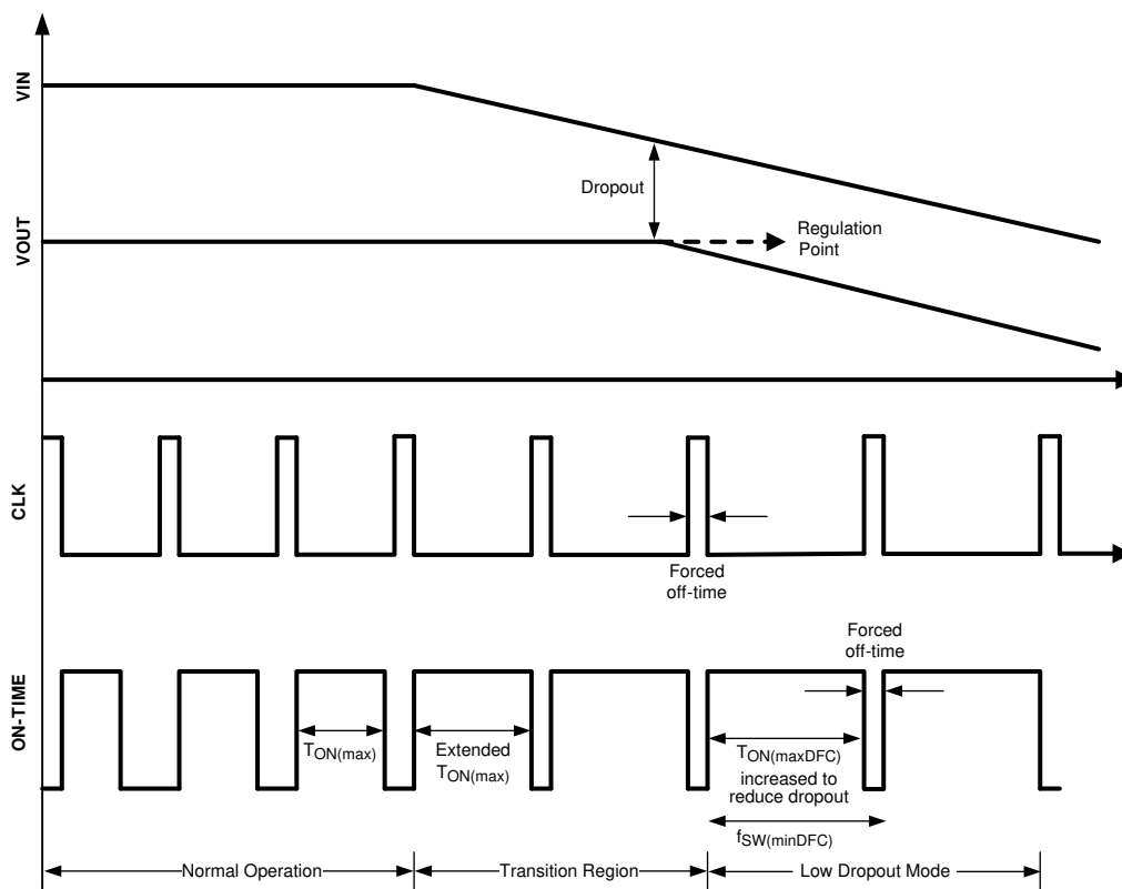
FIG 7-4. Dropout Voltage Reduction using Dynamic Frequency Control
