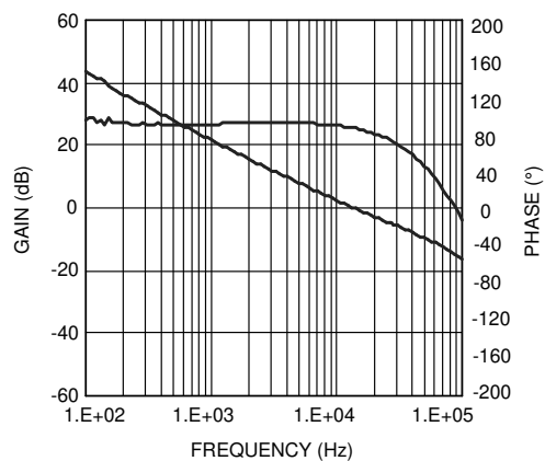
8-6. Overall Loop Gain and Phase
