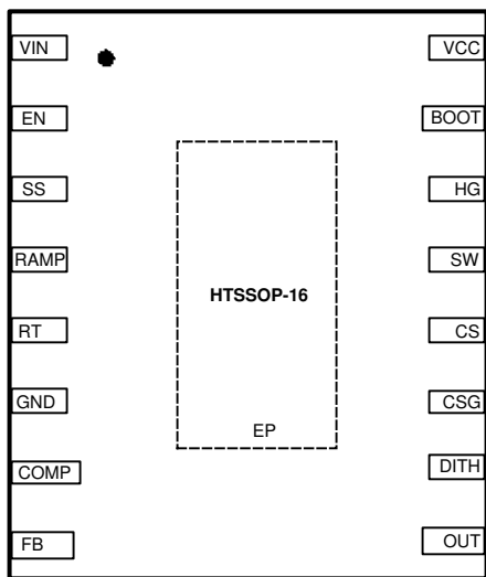
图 5-1. LM25088-1 16-Pin PWP Package (Dither Version) (Top View)
