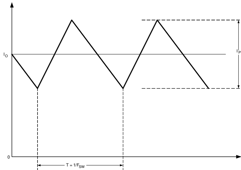
FIG 8-2. Inductor Current
