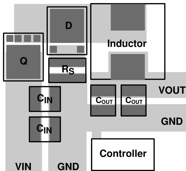
FIG 10-1. LM25088 Layout Example
