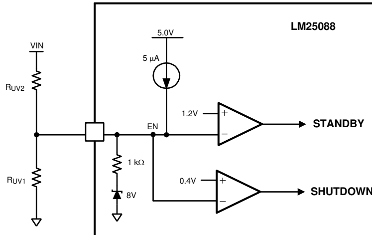
FIG 7-2. Basic Enable Configuration
