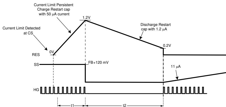
7-8. Current Limit Restart Timing Diagram
