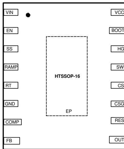
图 5-2. LM25088-2 16-Pin PWP Package (Restart Version) (Top View)
