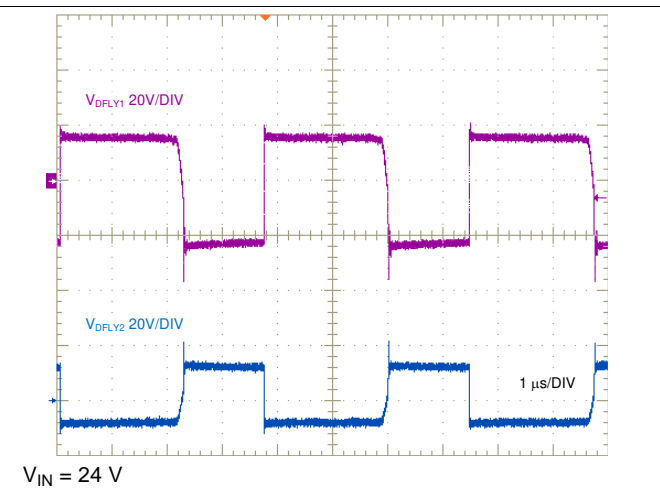
Figure 42. Flyback Diode Voltages, Full Load
