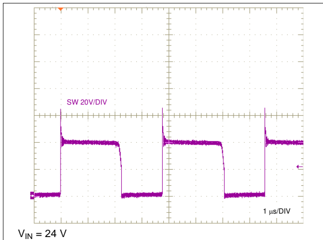
Figure 41. SW Node Voltage, Full Load
