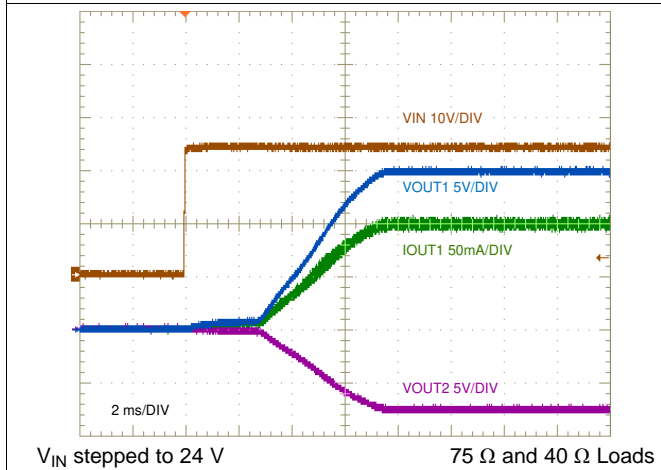
Figure 39. Start-Up Characteristic
