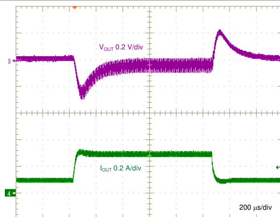
8-11. Load Transient, 0.1 A to 0.6 A, 0.1 A/ \mu s
