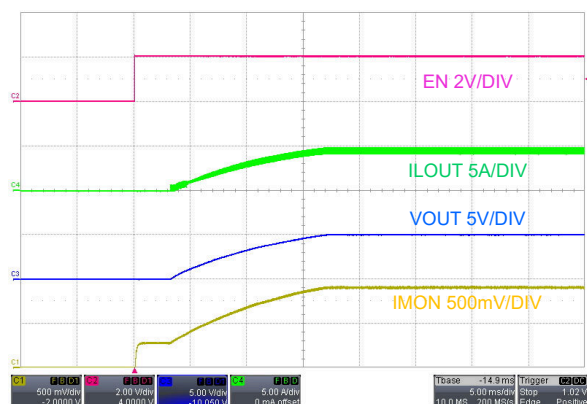
図 7-7. Start-Up, EN ON, V_{SUPPLY} = 12V , I_{LOAD} = 5A Resistive Load
