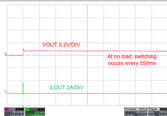
図 7-10. No Load Operation in PFM Mode, V_{SUPPLY} = 12V
