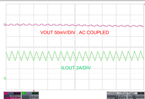
図 7-9. Output Ripple, V_{SUPPLY} = 12V
