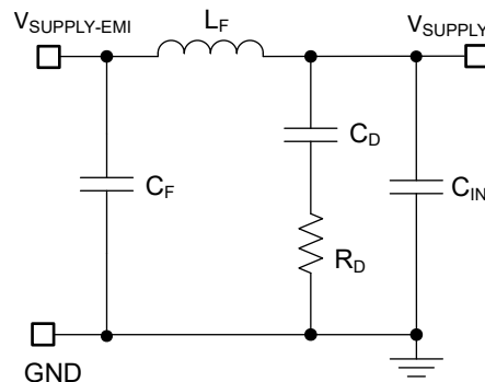
FIG 7-2. Passive π-Stage EMI Filter for Buck Regulator
