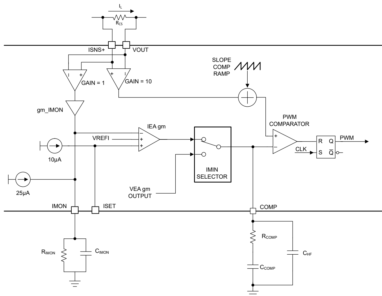
6-5. Current Loop Functional Block Diagram
