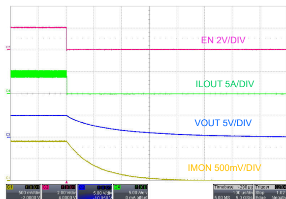
図 7-8. Shutdown, EN OFF, V_{SUPPLY} = 12V , I_{LOAD} = 5A Resistive Load
