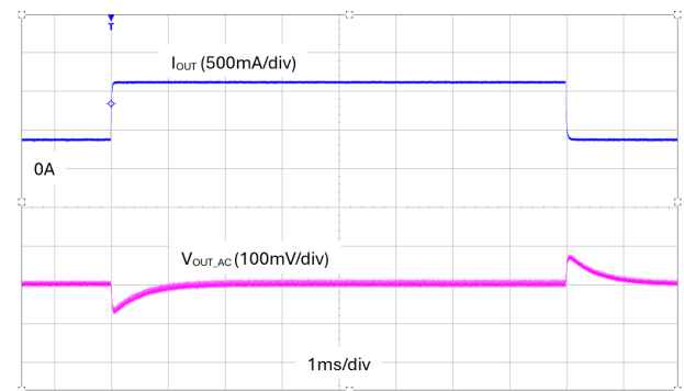
図 7-10. 負荷過渡応答 ( V_{IN} = 24V , V_{OUT} = 5V , I_{OUT} = 400mA \sim 1.2A )
