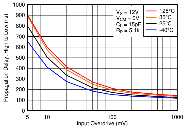
FIG 6-27. High to Low Propagation Delay vs. Input Overdrive Voltage, 12V
