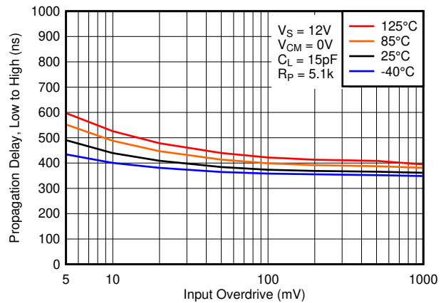
FIG 6-28. Low to High Propagation Delay vs. Input Overdrive Voltage, 12V
