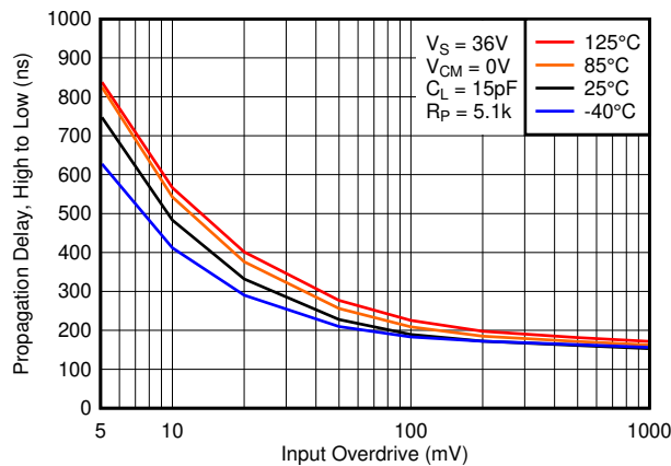
FIG 6-29. High to Low Propagation Delay vs. Input Overdrive Voltage, 36V
