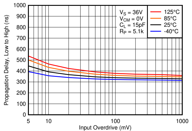
FIG 6-30. Low to High Propagation Delay vs. Input Overdrive Voltage, 36V
